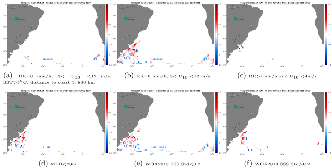
Figure 12: Temporal mean gridded over spatial boxes of size 1^{\circ}\times 1^{\circ} of \Delta\text{SSS} (SMOS SSS L3 v9 - 9 Days (CATDS-CEC-LOCEAN) - Marine mammals) for 6 different subdatasets corresponding to:RR=0 mm/h, 3 < U_{10} < 12 m/s, SST >5^{\circ}\text{C} , distance to coast > 800 km (a), RR=0 mm/h, 3 < U_{10} < 12 m/s (b), RR >1 mm/h and U_{10} < 4 m/s (c),MLD <20 m (d),WOA2013 SSS Std <0.2 (e),WOA2013 SSS Std >0.2 (f).
