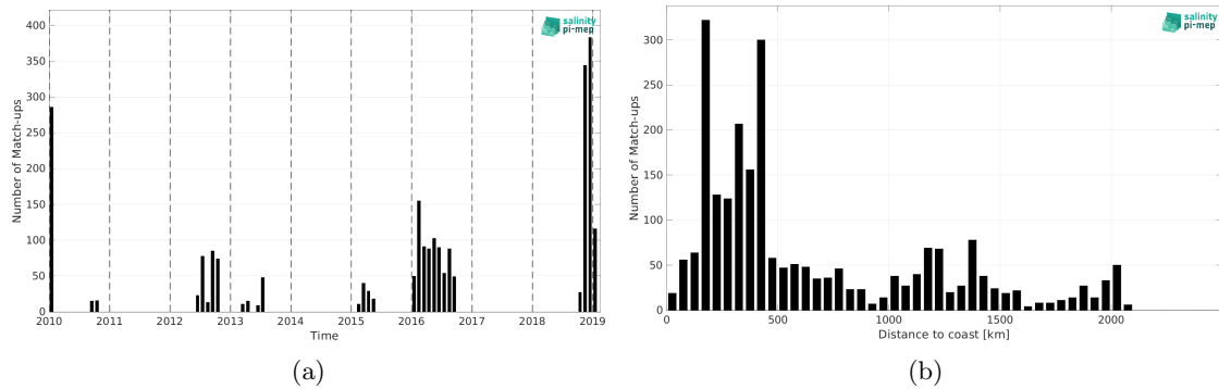
Figure 1: Number of match-ups between Marine mammals and SMOS SSS L3 v9 - 9 Days (CATDS-CEC-LOCEAN) SSS as a function of time (a) and as function of the distance to coast (b) over the South Atlantic Ocean Pi-MEP region and for the full satellite product period.
