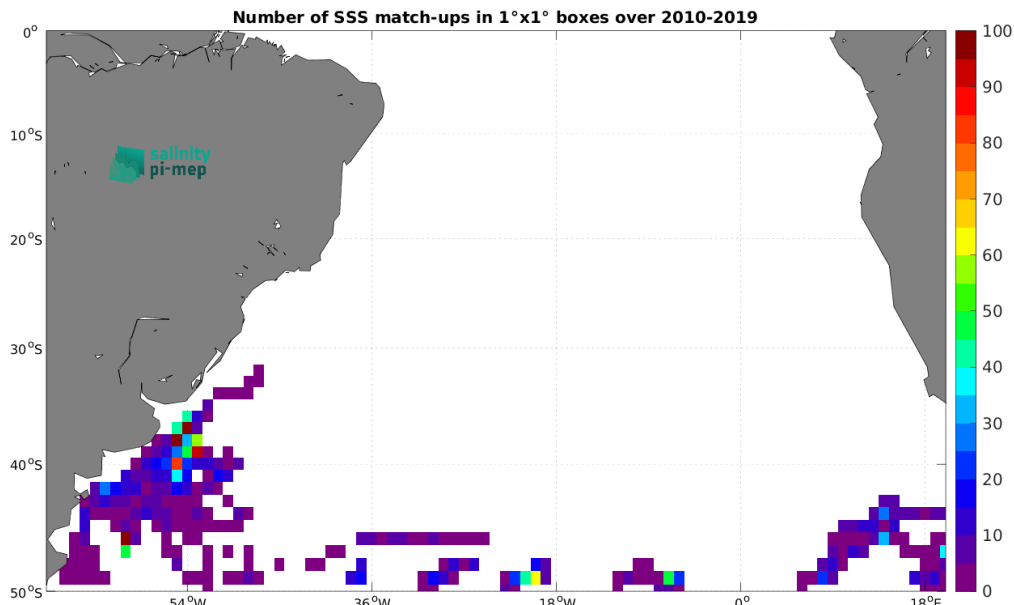
Figure 4: Number of SSS match-ups between Marine mammals SSS and the SMOS SSS L3 v9 - 9 Days (CATDS-CEC-LOCEAN) SSS product for the South Atlantic Ocean Pi-MEP region over 1^\circ \times 1^\circ boxes and for the full satellite product period.
