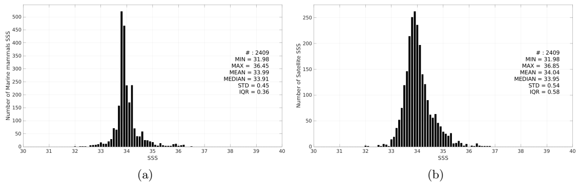
Figure 2: Histograms of SSS from Marine mammals (a) and SMOS SSS L3 v9 - 9 Days (CATDS-CEC-LOCEAN) (b) considering all match-up pairs per bins of 0.1 over the South Atlantic Ocean Pi-MEP region and for the full satellite product period.
