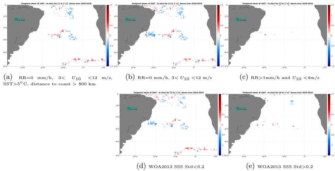
Figure 13: Temporal mean gridded over spatial boxes of size 1^\circ \times 1^\circ of \Delta\text{SSS} (SMOS SSS L3 v9 - 9 Days (CATDS-CEC-LOCEAN) - Surface drifters) for 5 different subdatasets corresponding to:RR=0 mm/h, 3 < U_{10} < 12 m/s, SST >5^\circ\text{C} , distance to coast > 800 km (a), RR=0 mm/h, 3 < U_{10} < 12 m/s (b), RR >1 mm/h and U_{10} < 4 m/s (c), WOA2013 SSS Std <0.2 (d), WOA2013 SSS Std >0.2 (e).
