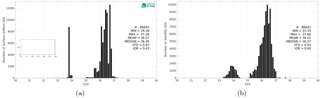
Figure 3: Histograms of SSS from Surface drifters (a) and SMOS SSS L3 v9 - 9 Days (CATDS-CEC-LOCEAN) (b) considering all match-up pairs per bins of 0.1 over the South Atlantic Ocean Pi-MEP region and for the full satellite product period.
