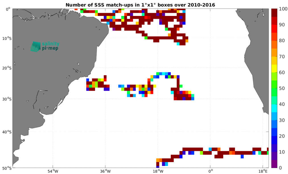
Figure 4: Number of SSS match-ups between Surface drifters SSS and the SMOS SSS L3 v9 - 9 Days (CATDS-CEC-LOCEAN) SSS product for the South Atlantic Ocean Pi-MEP region over 1^\circ \times 1^\circ boxes and for the full satellite product period.
