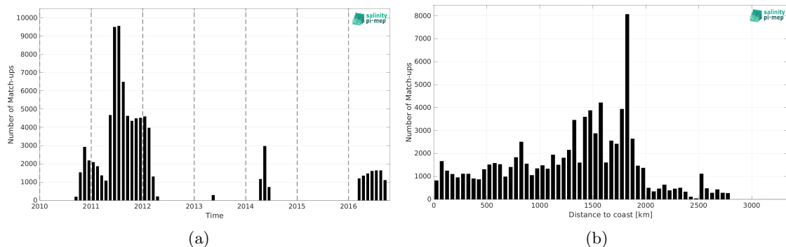
Figure 2: Number of match-ups between Surface drifters and SMOS SSS L3 v9 - 9 Days (CATDS-CEC-LOCEAN) SSS as a function of time (a) and as function of the distance to coast (b) over the South Atlantic Ocean Pi-MEP region and for the full satellite product period.
