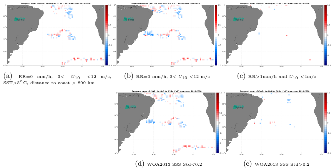
Figure 11: Temporal mean gridded over spatial boxes of size 1^\circ \times 1^\circ of \Delta SSS (SMOS SSS L3 v9 - 9 Days (CATDS-CEC-LOCEAN) - Surface drifters) for 5 different subdatasets corresponding to:RR=0 mm/h, 3 < U_{10} < 12 m/s, SST >5^\circ\text{C} , distance to coast > 800 km (a), RR=0 mm/h, 3 < U_{10} < 12 m/s (b), RR >1 mm/h and U_{10} < 4 m/s (c), WOA2013 SSS Std <0.2 (d), WOA2013 SSS Std >0.2 (e).
