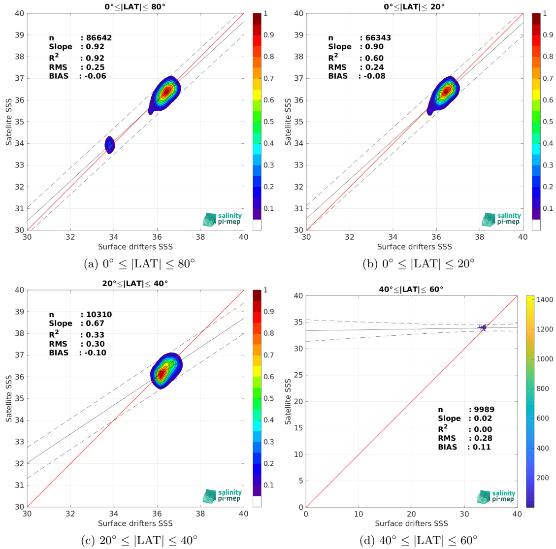
Figure 8: Contour maps of the concentration of SMOS SSS L3 v9 - 9 Days (CATDS-CEC-LOCEAN) SSS ( y -axis) versus Surface drifters SSS ( x -axis) at match-up pairs for different latitude bands. For each plot, the red line shows x=y . The black thin and dashed lines indicate a linear fit through the data cloud and the \pm 95\% confidence levels, respectively. The number match-up pairs n , the slope and R^2 coefficient of the linear fit, the root mean square (RMS) and the mean bias between satellite and in situ data are indicated for each latitude band in each plots.
