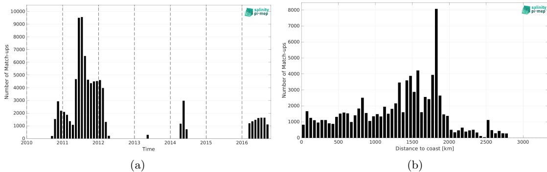
Figure 1: Number of match-ups between Surface drifters and SMOS SSS L3 v9 - 9 Days (CATDS-CEC-LOCEAN) SSS as a function of time (a) and as function of the distance to coast (b) over the South Atlantic Ocean Pi-MEP region and for the full satellite product period.
