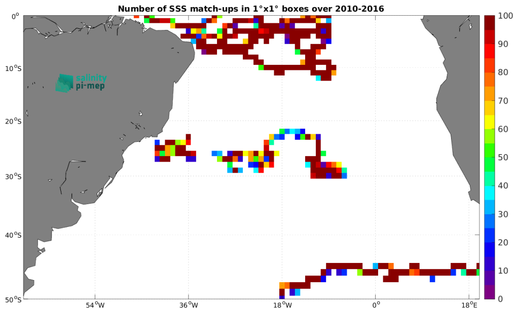
Figure 3: Number of SSS match-ups between Surface drifters SSS and the SMOS SSS L3 v9 - 9 Days (CATDS-CEC-LOCEAN) SSS product for the South Atlantic Ocean Pi-MEP region over 1^\circ \times 1^\circ boxes and for the full satellite product period.
