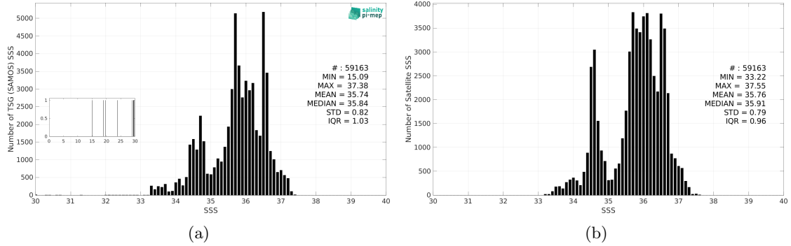
Figure 3: Histograms of SSS from TSG (SAMOS) (a) and SMOS SSS L3 v9 - 18 Days (CATDS-CEC-LOCEAN) (b) considering all match-up pairs per bins of 0.1 over the South Atlantic Ocean Pi-MEP region and for the full satellite product period.
