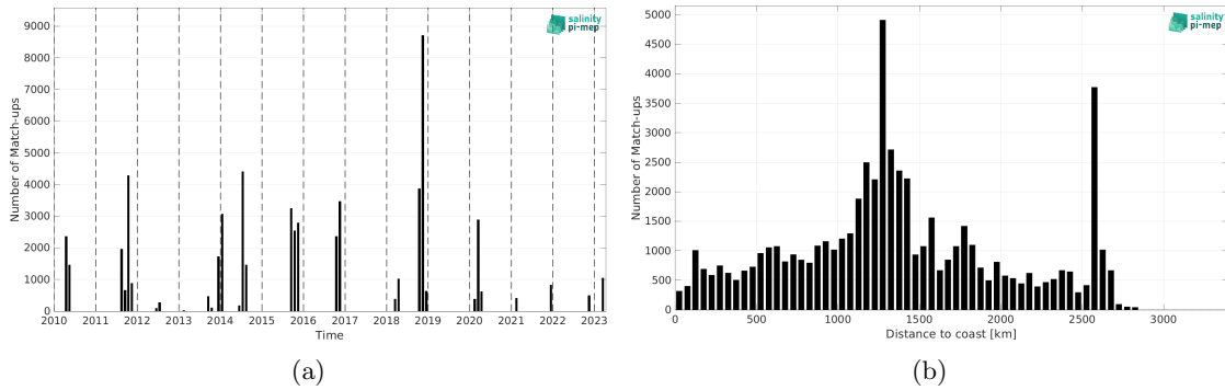
Figure 2: Number of match-ups between TSG (SAMOS) and SMOS SSS L3 v9 - 18 Days (CATDS-CEC-LOCEAN) SSS as a function of time (a) and as function of the distance to coast (b) over the South Atlantic Ocean Pi-MEP region and for the full satellite product period.
