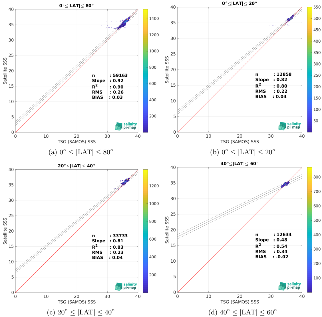
Figure 10: Contour maps of the concentration of SMOS SSS L3 v9 - 18 Days (CATDS-CEC-LOCEAN) SSS (y-axis) versus TSG (SAMOS) SSS (x-axis) at match-up pairs for different latitude bands. For each plot, the red line shows x=y . The black thin and dashed lines indicate a linear fit through the data cloud and the \pm 95\% confidence levels, respectively. The number match-up pairs n , the slope and R^2 coefficient of the linear fit, the root mean square (RMS) and the mean bias between satellite and in situ data are indicated for each latitude band in each plots.
