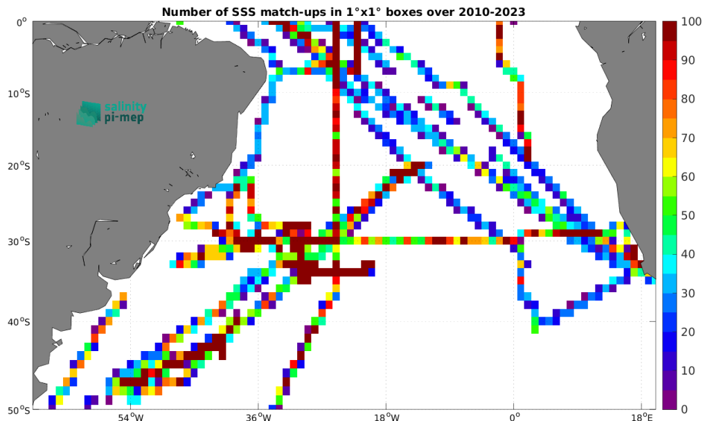
Figure 4: Number of SSS match-ups between TSG (SAMOS) SSS and the SMOS SSS L3 v9 - 18 Days (CATDS-CEC-LOCEAN) SSS product for the South Atlantic Ocean Pi-MEP region over 1^\circ \times 1^\circ boxes and for the full satellite product period.
