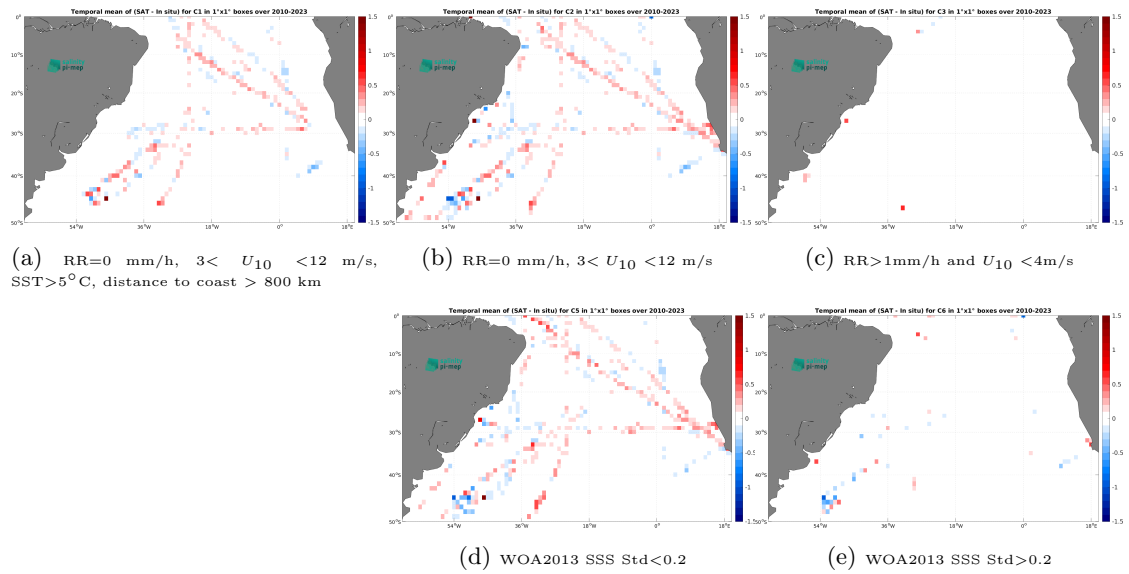
Figure 12: Temporal mean gridded over spatial boxes of size 1^\circ \times 1^\circ of \Delta SSS (SMOS SSS L3 v9 - 18 Days (CATDS-CEC-LOCEAN) - TSG (SAMOS)) for 5 different subdatasets corresponding to:RR=0 mm/h, 3 < U_{10} < 12 m/s, SST >5^\circ\text{C} , distance to coast > 800 km (a), RR=0 mm/h, 3 < U_{10} < 12 m/s (b), RR >1 mm/h and U_{10} < 4 m/s (c), WOA2013 SSS Std <0.2 (d), WOA2013 SSS Std >0.2 (e).
