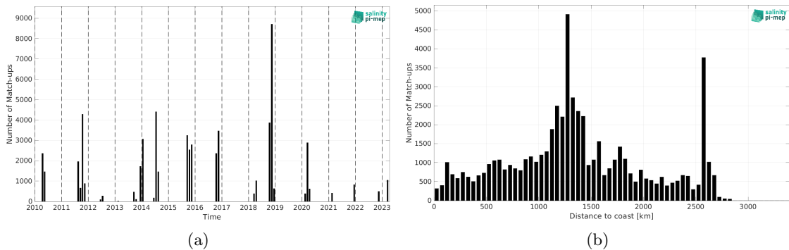
Figure 1: Number of match-ups between TSG (SAMOS) and SMOS SSS L3 v9 - 18 Days (CATDS-CEC-LOCEAN) SSS as a function of time (a) and as function of the distance to coast (b) over the South Atlantic Ocean Pi-MEP region and for the full satellite product period.
