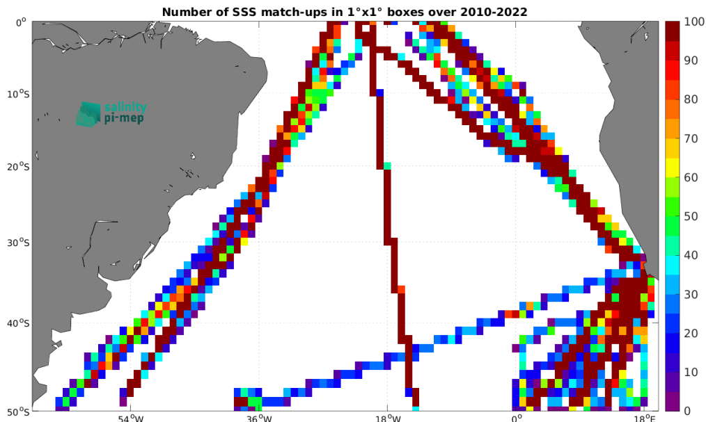
Figure 4: Number of SSS match-ups between TSG (Polarstern) SSS and the SMOS SSS L3 v9 - 18 Days (CATDS-CEC-LOCEAN) SSS product for the South Atlantic Ocean Pi-MEP region over 1^\circ \times 1^\circ boxes and for the full satellite product period.
