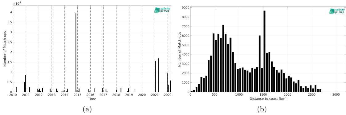
Figure 1: Number of match-ups between TSG (Polarstern) and SMOS SSS L3 v9 - 18 Days (CATDS-CEC-LOCEAN) SSS as a function of time (a) and as function of the distance to coast (b) over the South Atlantic Ocean Pi-MEP region and for the full satellite product period.
