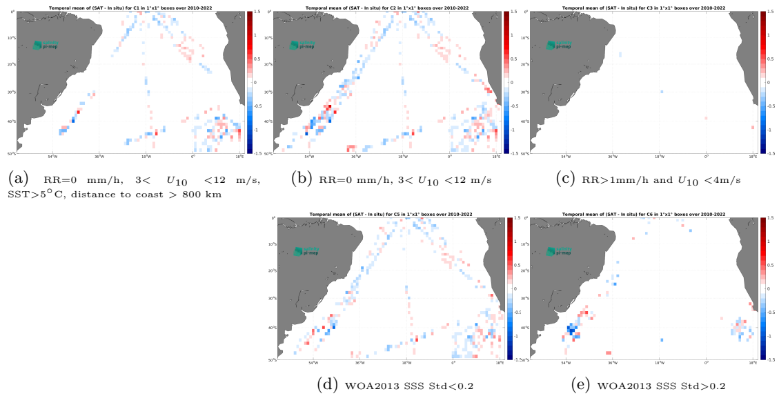
Figure 12: Temporal mean gridded over spatial boxes of size 1^\circ \times 1^\circ of \Delta SSS (SMOS SSS L3 v9 - 18 Days (CATDS-CEC-LOCEAN) - TSG (Polarstern)) for 5 different subdatasets corresponding to:RR=0 mm/h, 3 < U_{10} < 12 m/s, SST >5^\circ\text{C} , distance to coast > 800 km (a), RR=0 mm/h, 3 < U_{10} < 12 m/s (b), RR >1 mm/h and U_{10} < 4 m/s (c), WOA2013 SSS Std <0.2 (d), WOA2013 SSS Std >0.2 (e).
