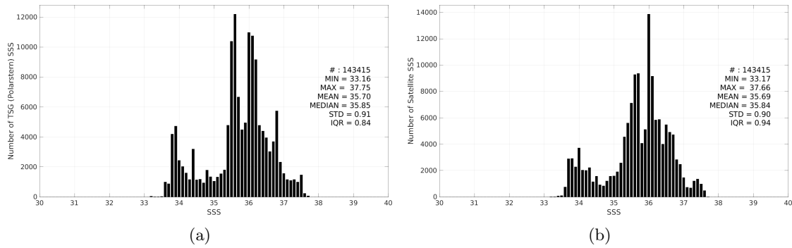
Figure 2: Histograms of SSS from TSG (Polarstern) (a) and SMOS SSS L3 v9 - 18 Days (CATDS-CEC-LOCEAN) (b) considering all match-up pairs per bins of 0.1 over the South Atlantic Ocean Pi-MEP region and for the full satellite product period.
