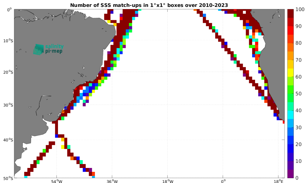
Figure 5: Number of SSS match-ups between TSG (LEGOS-DM) SSS and the SMOS SSS L3 v9 - 18 Days (CATDS-CEC-LOCEAN) SSS product for the South Atlantic Ocean Pi-MEP region over 1^\circ \times 1^\circ boxes and for the full satellite product period.
