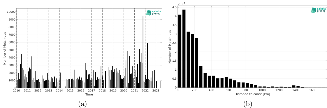
Figure 2: Number of match-ups between TSG (LEGOS-DM) and SMOS SSS L3 v9 - 18 Days (CATDS-CEC-LOCEAN) SSS as a function of time (a) and as function of the distance to coast (b) over the South Atlantic Ocean Pi-MEP region and for the full satellite product period.
