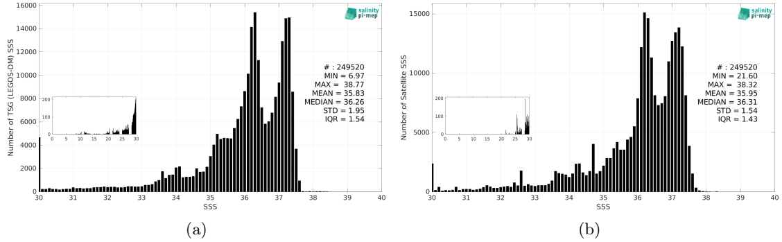
Figure 3: Histograms of SSS from TSG (LEGOS-DM) (a) and SMOS SSS L3 v9 - 18 Days (CATDS-CEC-LOCEAN) (b) considering all match-up pairs per bins of 0.1 over the South Atlantic Ocean Pi-MEP region and for the full satellite product period.
