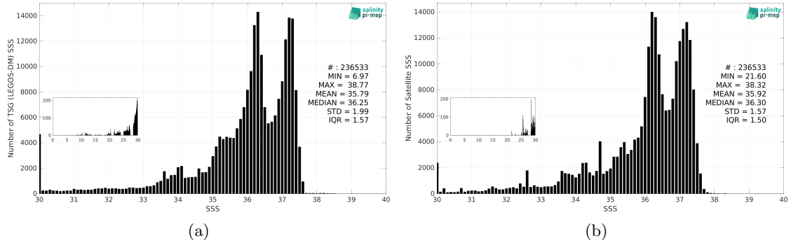
Figure 3: Histograms of SSS from TSG (LEGOS-DM) (a) and SMOS SSS L3 v9 - 18 Days (CATDS-CEC-LOCEAN) (b) considering all match-up pairs per bins of 0.1 over the South Atlantic Ocean Pi-MEP region and for the full satellite product period.
