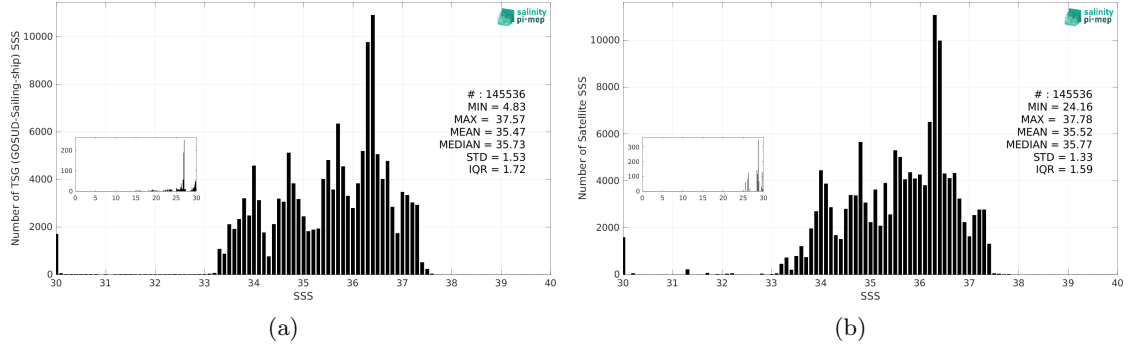
Figure 3: Histograms of SSS from TSG (GOSUD-Sailing-ship) (a) and SMOS SSS L3 v9 - 18 Days (CATDS-CEC-LOCEAN) (b) considering all match-up pairs per bins of 0.1 over the South Atlantic Ocean Pi-MEP region and for the full satellite product period.
