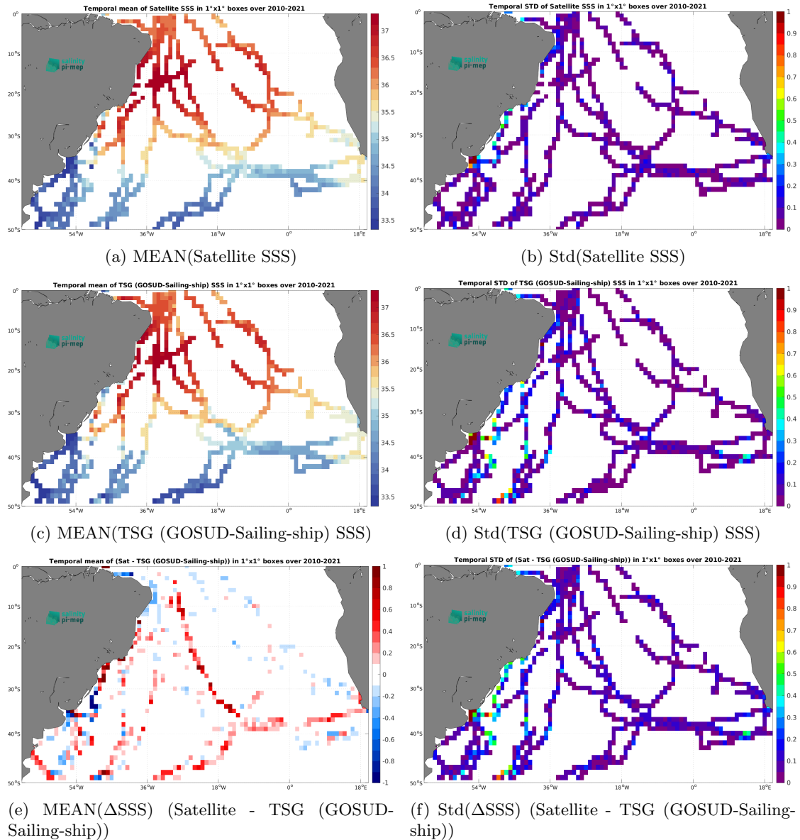
Figure 7: Temporal mean (left) and Std (right) of SSS from SMOS SSS L3 v9 - 18 Days (CATDS-CEC-LOCEAN) (top), TSG (GOSUD-Sailing-ship) (middle), and of \Delta SSS (Satellite - TSG (GOSUD-Sailing-ship)). Only match-up pairs are used to generate these maps.
