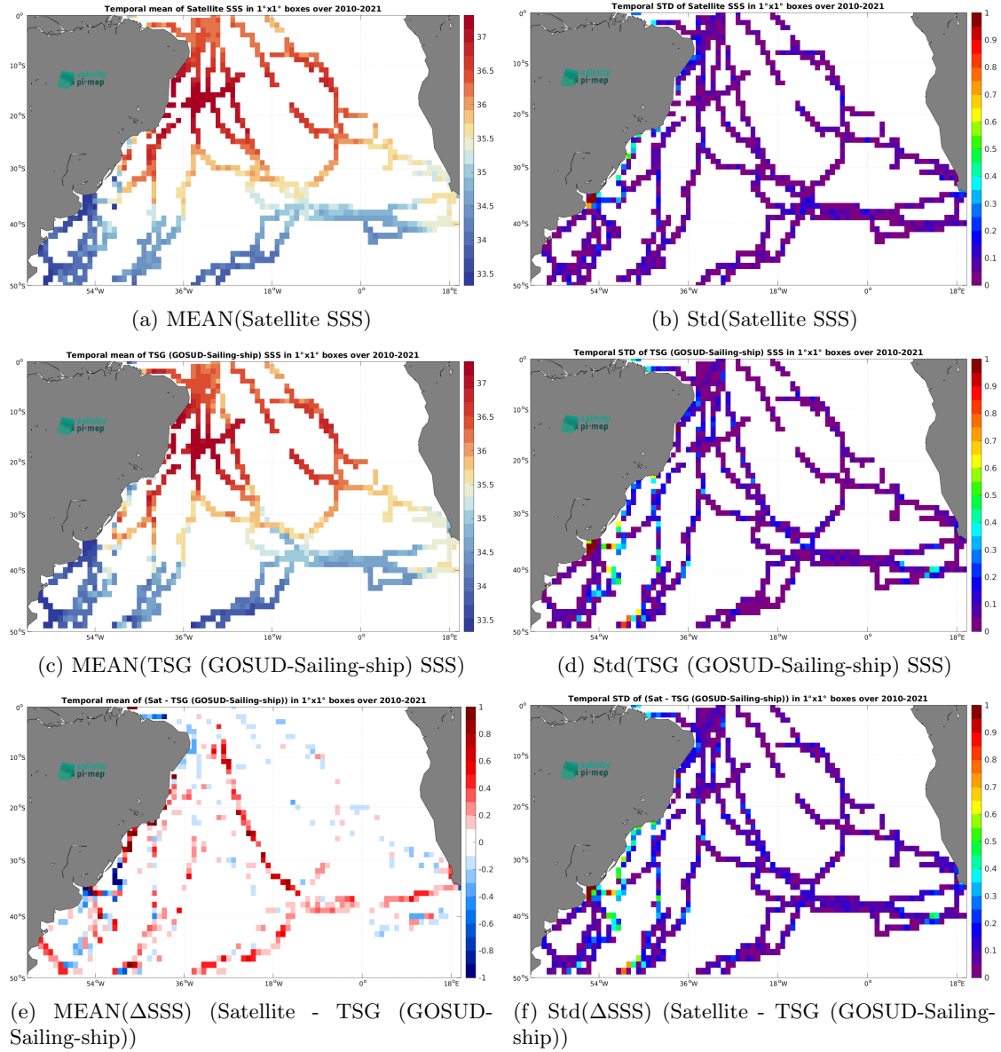
Figure 6: Temporal mean (left) and Std (right) of SSS from SMOS SSS L3 v9 - 18 Days (CATDS-CEC-LOCEAN) (top), TSG (GOSUD-Sailing-ship) (middle), and of \Delta SSS (Satellite - TSG (GOSUD-Sailing-ship)). Only match-up pairs are used to generate these maps.
