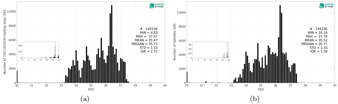
Figure 2: Histograms of SSS from TSG (GOSUD-Sailing-ship) (a) and SMOS SSS L3 v9 - 18 Days (CATDS-CEC-LOCEAN) (b) considering all match-up pairs per bins of 0.1 over the South Atlantic Ocean Pi-MEP region and for the full satellite product period.
