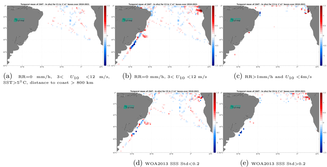
Figure 14: Temporal mean gridded over spatial boxes of size 1^\circ \times 1^\circ of \Delta\text{SSS} (SMOS SSS L3 v9 - 18 Days (CATDS-CEC-LOCEAN) - TSG (GOSUD-Research-vessel)) for 5 different subdatasets corresponding to:RR=0 mm/h, 3 < U_{10} < 12 m/s, SST >5^\circ\text{C} , distance to coast > 800 km (a), RR=0 mm/h, 3 < U_{10} < 12 m/s (b), RR >1 mm/h and U_{10} < 4 m/s (c), WOA2013 SSS Std <0.2 (d), WOA2013 SSS Std >0.2 (e).
