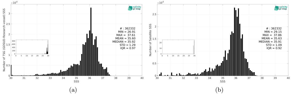
Figure 3: Histograms of SSS from TSG (GOSUD-Research-vessel) (a) and SMOS SSS L3 v9 - 18 Days (CATDS-CEC-LOCEAN) (b) considering all match-up pairs per bins of 0.1 over the South Atlantic Ocean Pi-MEP region and for the full satellite product period.
