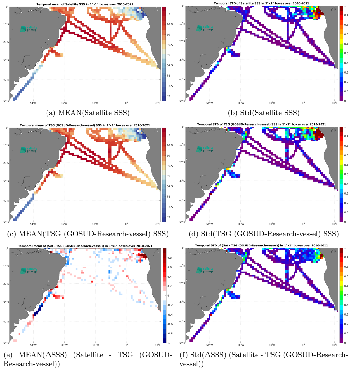
Figure 7: Temporal mean (left) and Std (right) of SSS from SMOS SSS L3 v9 - 18 Days (CATDS-CEC-LOCEAN) (top), TSG (GOSUD-Research-vessel) (middle), and of \Delta SSS (Satellite - TSG (GOSUD-Research-vessel)). Only match-up pairs are used to generate these maps.
