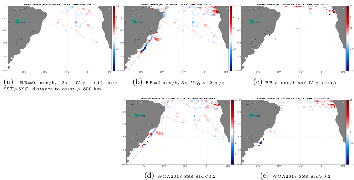
Figure 12: Temporal mean gridded over spatial boxes of size 1^\circ \times 1^\circ of \Delta\text{SSS} (SMOS SSS L3 v9 - 18 Days (CATDS-CEC-LOCEAN) - TSG (GOSUD-Research-vessel)) for 5 different subdatasets corresponding to:RR=0 mm/h, 3 < U_{10} < 12 m/s, SST >5^\circ\text{C} , distance to coast > 800 km (a), RR=0 mm/h, 3 < U_{10} < 12 m/s (b), RR >1 mm/h and U_{10} < 4 m/s (c), WOA2013 SSS Std <0.2 (d), WOA2013 SSS Std >0.2 (e).
