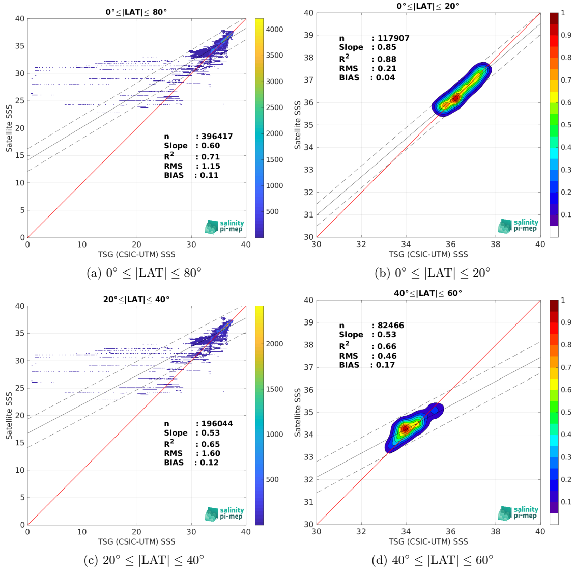
Figure 10: Contour maps of the concentration of SMOS SSS L3 v9 - 18 Days (CATDS-CEC-LOCEAN) SSS ( y -axis) versus TSG (CSIC-UTM) SSS ( x -axis) at match-up pairs for different latitude bands. For each plot, the red line shows x=y . The black thin and dashed lines indicate a linear fit through the data cloud and the \pm 95\% confidence levels, respectively. The number match-up pairs n , the slope and R^2 coefficient of the linear fit, the root mean square (RMS) and the mean bias between satellite and in situ data are indicated for each latitude band in each plots.
