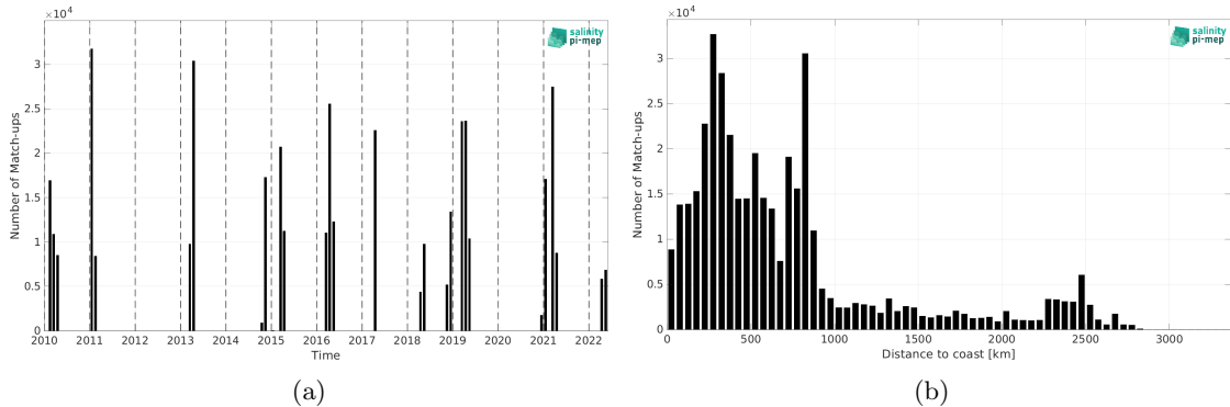
Figure 2: Number of match-ups between TSG (CSIC-UTM) and SMOS SSS L3 v9 - 18 Days (CATDS-CEC-LOCEAN) SSS as a function of time (a) and as function of the distance to coast (b) over the South Atlantic Ocean Pi-MEP region and for the full satellite product period.
