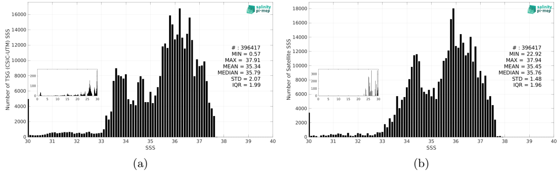
Figure 3: Histograms of SSS from TSG (CSIC-UTM) (a) and SMOS SSS L3 v9 - 18 Days (CATDS-CEC-LOCEAN) (b) considering all match-up pairs per bins of 0.1 over the South Atlantic Ocean Pi-MEP region and for the full satellite product period.
