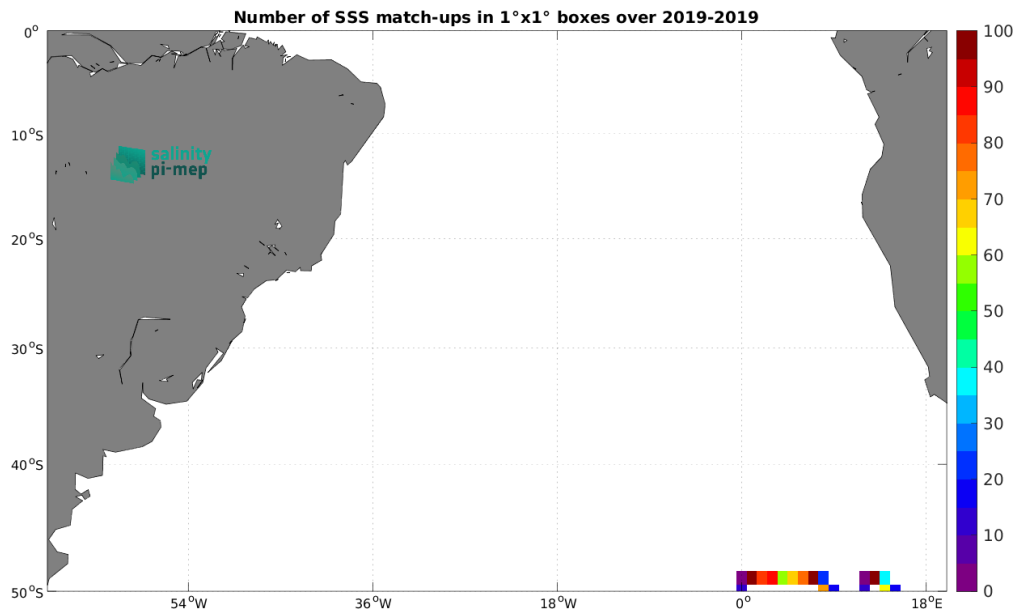
Figure 5: Number of SSS match-ups between Sairdrone SSS and the SMOS SSS L3 v9 - 18 Days (CATDS-CEC-LOCEAN) SSS product for the South Atlantic Ocean Pi-MEP region over 1^\circ \times 1^\circ boxes and for the full satellite product period.
