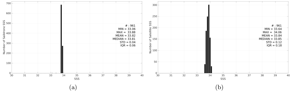
Figure 3: Histograms of SSS from Saildrone (a) and SMOS SSS L3 v9 - 18 Days (CATDS-CEC-LOCEAN) (b) considering all match-up pairs per bins of 0.1 over the South Atlantic Ocean Pi-MEP region and for the full satellite product period.
