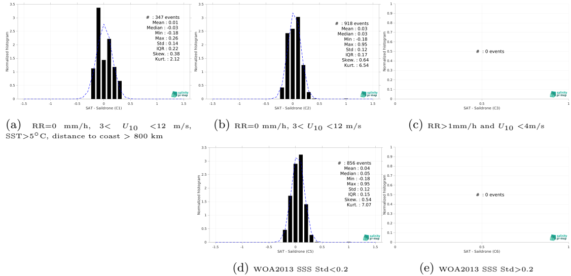
Figure 15: Normalized histogram of \Delta SSS (SMOS SSS L3 v9 - 18 Days (CATDS-CEC-LOCEAN) - Saildrone) for 5 different subdatasets corresponding to: RR=0 mm/h, 3 < U_{10} < 12 m/s, SST > 5°C, distance to coast > 800 km (a), RR=0 mm/h, 3 < U_{10} < 12 m/s (b), RR > 1mm/h and U_{10} < 4 m/s (c), WOA2013 SSS Std < 0.2 (d), WOA2013 SSS Std > 0.2 (e).
