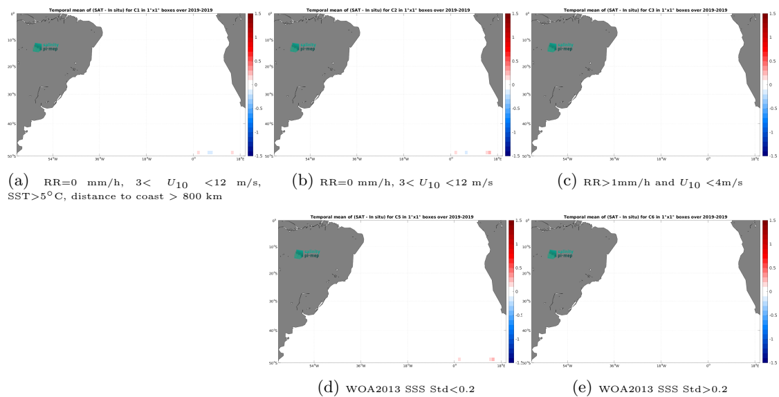
Figure 14: Temporal mean gridded over spatial boxes of size 1^\circ \times 1^\circ of \Delta SSS (SMOS SSS L3 v9 - 18 Days (CATDS-CEC-LOCEAN) - Sailydrone) for 5 different subdatasets corresponding to:RR=0 mm/h, 3 < U_{10} < 12 m/s, SST >5^\circ C, distance to coast > 800 km (a), RR=0 mm/h, 3 < U_{10} < 12 m/s (b), RR >1 mm/h and U_{10} < 4 m/s (c), WOA2013 SSS Std <0.2 (d), WOA2013 SSS Std >0.2 (e).
