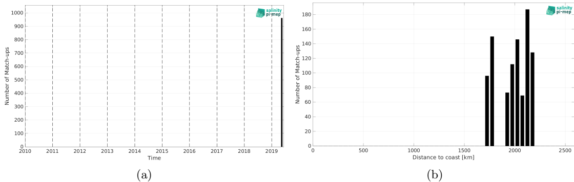
Figure 2: Number of match-ups between Saildrone and SMOS SSS L3 v9 - 18 Days (CATDS-CEC-LOCEAN) SSS as a function of time (a) and as function of the distance to coast (b) over the South Atlantic Ocean Pi-MEP region and for the full satellite product period.
