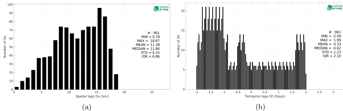
Figure 5: Histograms of the spatial (a) and temporal (b) lags between the location/time of the Sairdrone measurement and the date of the corresponding SMOS SSS L3 v9 - 18 Days (CATDS-CEC-LOCEAN) SSS pixel.
