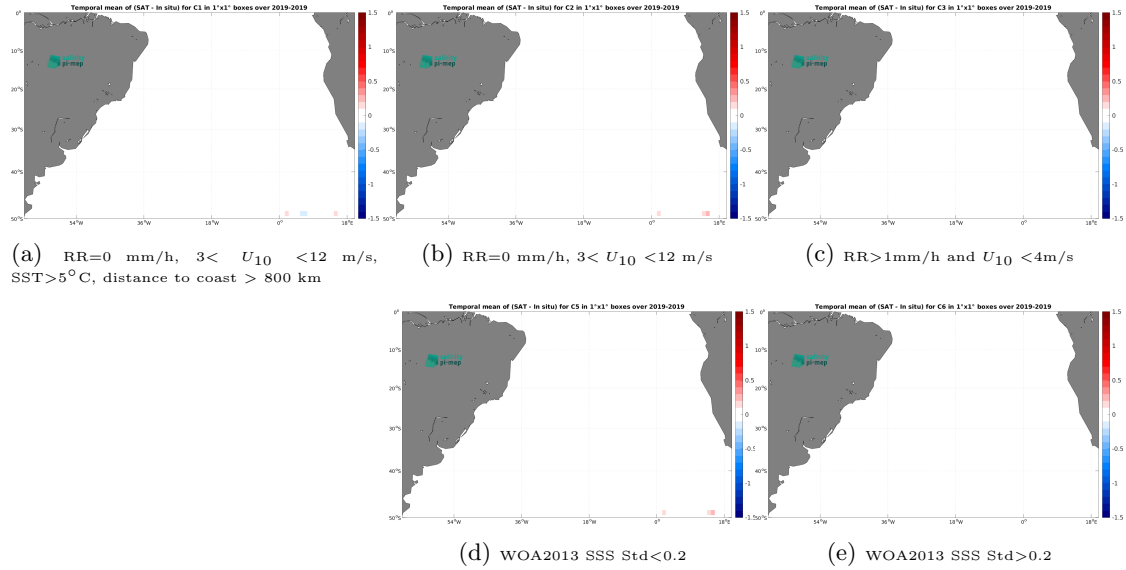
Figure 12: Temporal mean gridded over spatial boxes of size 1^{\circ}\times 1^{\circ} of \Delta\text{SSS} (SMOS SSS L3 v9 - 18 Days (CATDS-CEC-LOCEAN) - Saildrone) for 5 different subdatasets corresponding to:RR=0 mm/h, 3 < U_{10} < 12 m/s, SST >5^{\circ}\text{C} , distance to coast > 800 km (a), RR=0 mm/h, 3 < U_{10} < 12 m/s (b), RR >1 mm/h and U_{10} < 4 m/s (c), WOA2013 SSS Std <0.2 (d), WOA2013 SSS Std >0.2 (e).
