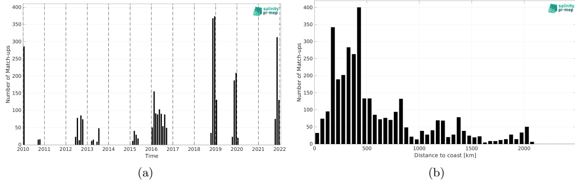
Figure 2: Number of match-ups between Marine mammals and SMOS SSS L3 v9 - 18 Days (CATDS-CEC-LOCEAN) SSS as a function of time (a) and as function of the distance to coast (b) over the South Atlantic Ocean Pi-MEP region and for the full satellite product period.
