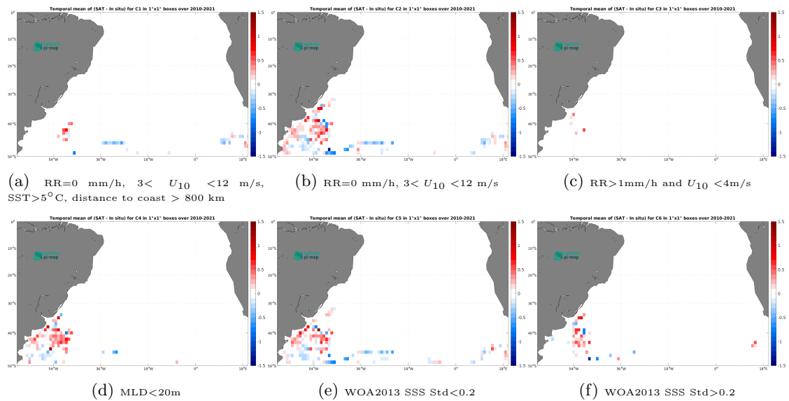
Figure 14: Temporal mean gridded over spatial boxes of size 1^\circ \times 1^\circ of \Delta SSS (SMOS SSS L3 v9 - 18 Days (CATDS-CEC-LOCEAN) - Marine mammals) for 6 different subdatasets corresponding to:RR=0 mm/h, 3 < U_{10} < 12 m/s, SST>5°C, distance to coast > 800 km (a), RR=0 mm/h, 3 < U_{10} < 12 m/s (b), RR>1mm/h and U_{10} < 4 m/s (c),MLD<20m (d),WOA2013 SSS Std<0.2 (e),WOA2013 SSS Std>0.2 (f).
