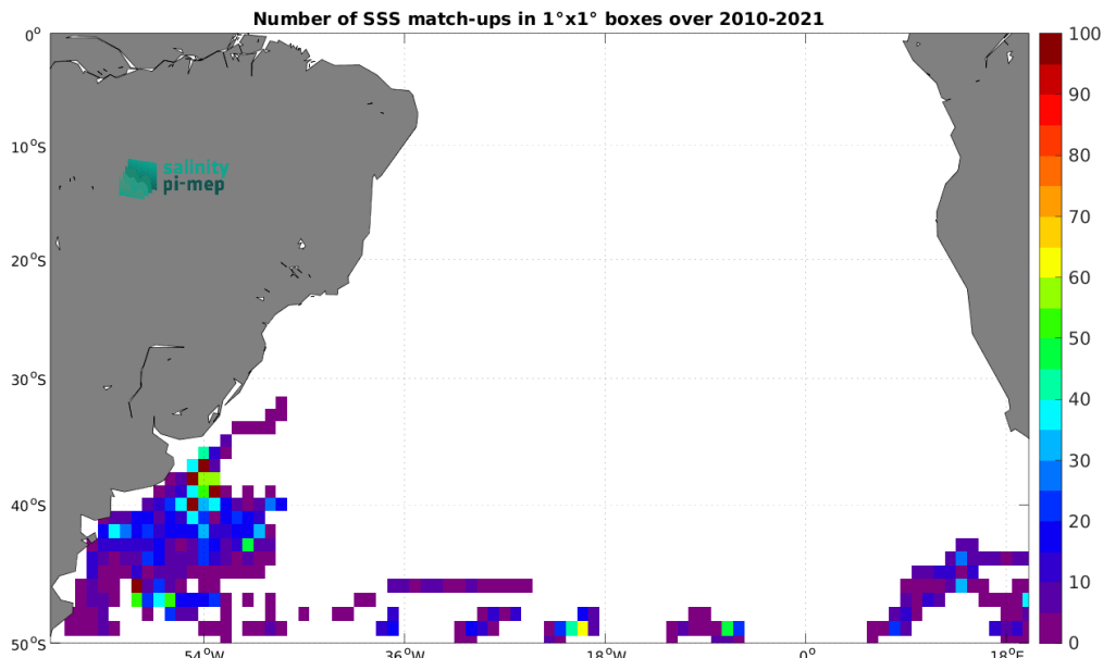
Figure 5: Number of SSS match-ups between Marine mammals SSS and the SMOS SSS L3 v9 - 18 Days (CATDS-CEC-LOCEAN) SSS product for the South Atlantic Ocean Pi-MEP region over 1^\circ \times 1^\circ boxes and for the full satellite product period.
