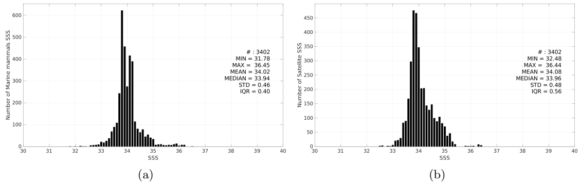
Figure 3: Histograms of SSS from Marine mammals (a) and SMOS SSS L3 v9 - 18 Days (CATDS-CEC-LOCEAN) (b) considering all match-up pairs per bins of 0.1 over the South Atlantic Ocean Pi-MEP region and for the full satellite product period.
