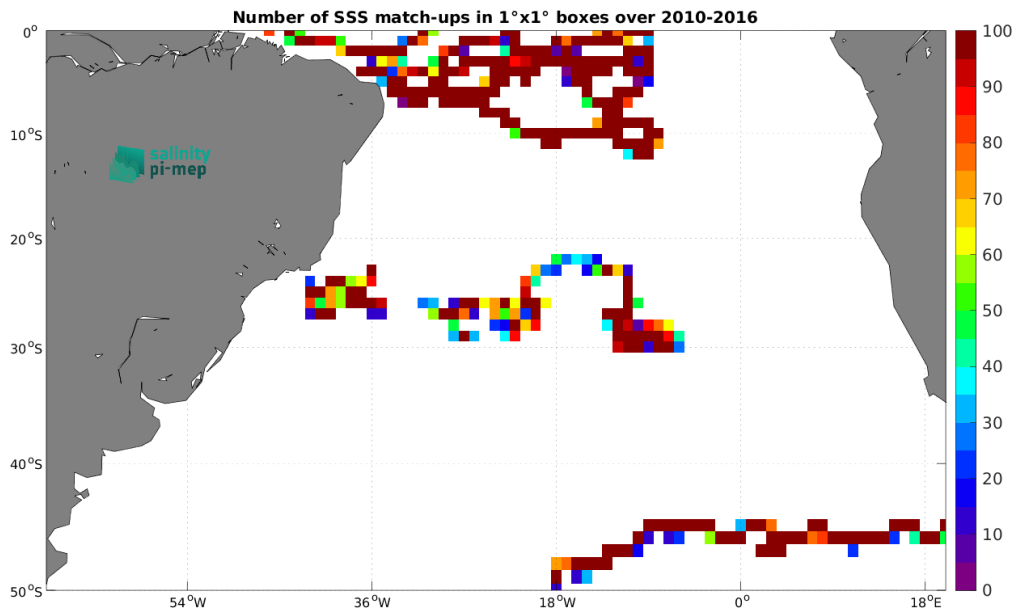
Figure 3: Number of SSS match-ups between Surface drifters SSS and the SMOS SSS L3 v9 - 18 Days (CATDS-CEC-LOCEAN) SSS product for the South Atlantic Ocean Pi-MEP region over 1^\circ \times 1^\circ boxes and for the full satellite product period.
