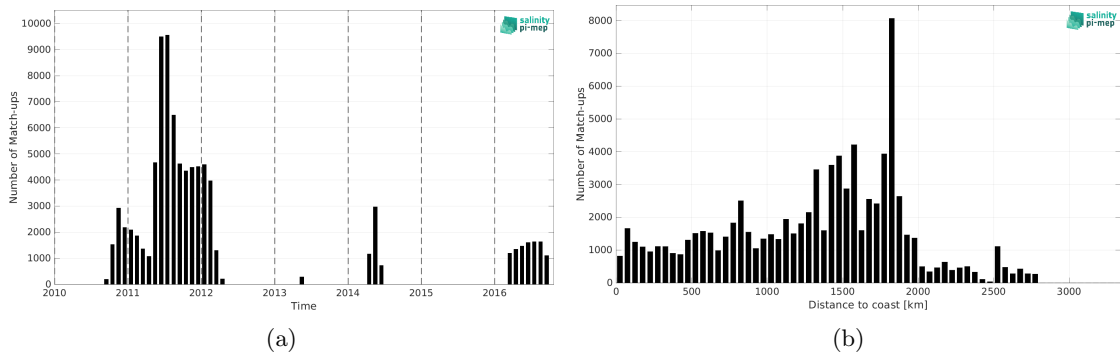
Figure 1: Number of match-ups between Surface drifters and SMOS SSS L3 v9 - 18 Days (CATDS-CEC-LOCEAN) SSS as a function of time (a) and as function of the distance to coast (b) over the South Atlantic Ocean Pi-MEP region and for the full satellite product period.
