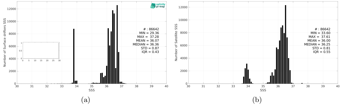
Figure 2: Histograms of SSS from Surface drifters (a) and SMOS SSS L3 v9 - 18 Days (CATDS-CEC-LOCEAN) (b) considering all match-up pairs per bins of 0.1 over the South Atlantic Ocean Pi-MEP region and for the full satellite product period.
