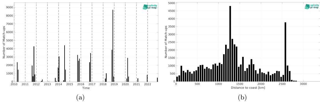
Figure 1: Number of match-ups between TSG (SAMOS) and SMOS SSS L3 v8 - 9 Days (CATDS-CEC-LOCEAN) SSS as a function of time (a) and as function of the distance to coast (b) over the South Atlantic Ocean Pi-MEP region and for the full satellite product period.
