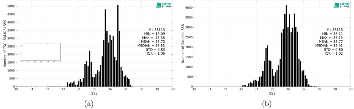
Figure 2: Histograms of SSS from TSG (SAMOS) (a) and SMOS SSS L3 v8 - 9 Days (CATDS-CEC-LOCEAN) (b) considering all match-up pairs per bins of 0.1 over the South Atlantic Ocean Pi-MEP region and for the full satellite product period.
