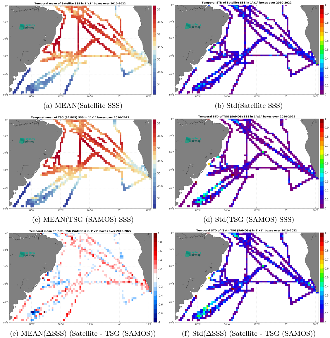
Figure 6: Temporal mean (left) and Std (right) of SSS from SMOS SSS L3 v8 - 9 Days (CATDS-CEC-LOCEAN) (top), TSG (SAMOS) (middle), and of \Delta SSS (Satellite - TSG (SAMOS)). Only match-up pairs are used to generate these maps.
