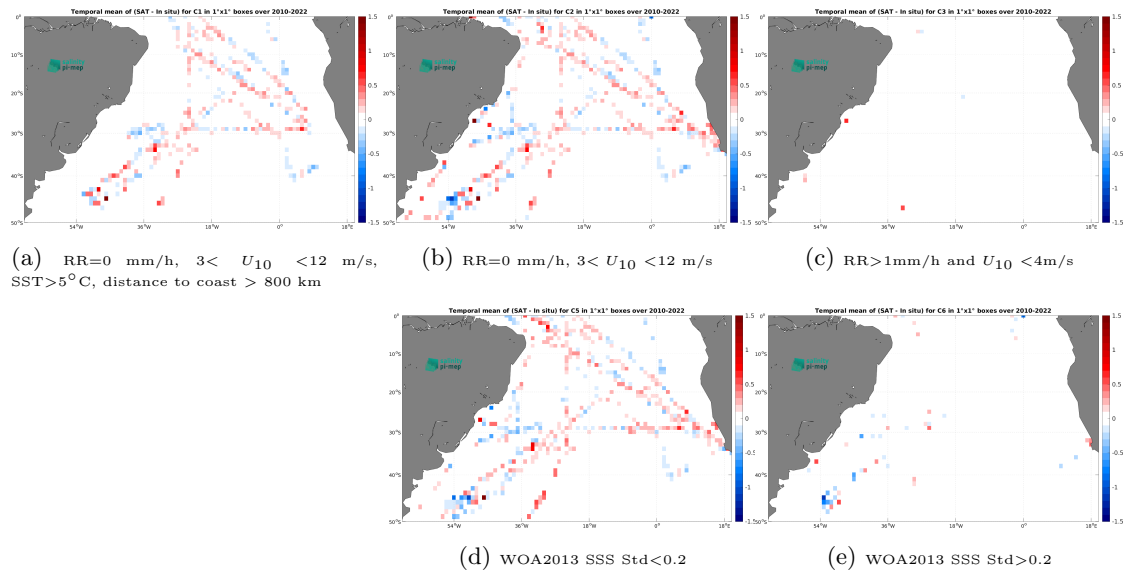
Figure 12: Temporal mean gridded over spatial boxes of size 1^\circ \times 1^\circ of \Delta SSS (SMOS SSS L3 v8 - 9 Days (CATDS-CEC-LOCEAN) - TSG (SAMOS)) for 5 different subdatasets corresponding to:RR=0 mm/h, 3 < U_{10} < 12 m/s, SST >5^\circ\text{C} , distance to coast > 800 km (a), RR=0 mm/h, 3 < U_{10} < 12 m/s (b), RR >1 mm/h and U_{10} < 4 m/s (c), WOA2013 SSS Std <0.2 (d), WOA2013 SSS Std >0.2 (e).
