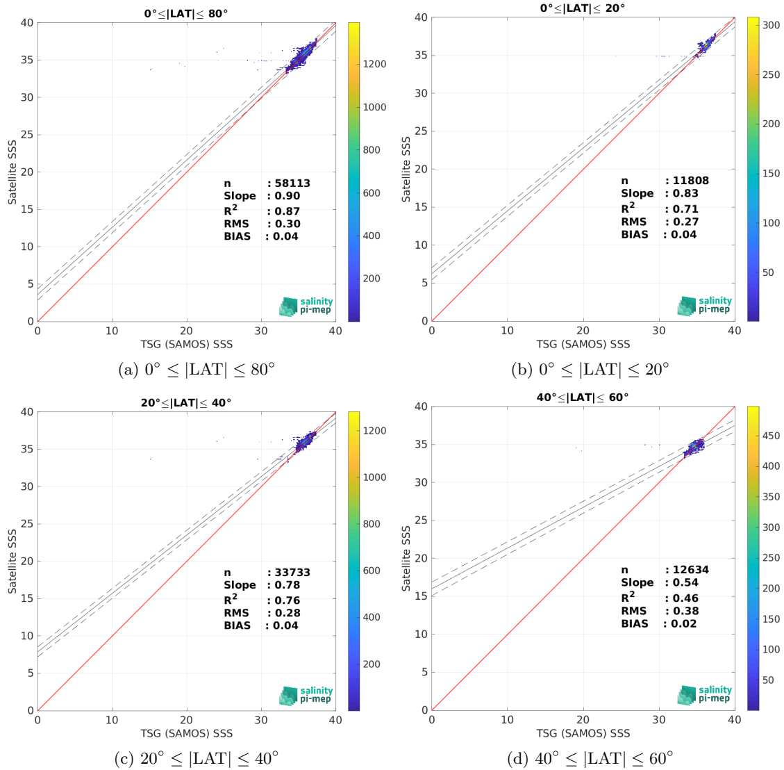
Figure 9: Contour maps of the concentration of SMOS SSS L3 v8 - 9 Days (CATDS-CEC-LOCEAN) SSS (y-axis) versus TSG (SAMOS) SSS (x-axis) at match-up pairs for different latitude bands. For each plot, the red line shows x=y . The black thin and dashed lines indicate a linear fit through the data cloud and the \pm 95\% confidence levels, respectively. The number match-up pairs n , the slope and R^2 coefficient of the linear fit, the root mean square (RMS) and the mean bias between satellite and in situ data are indicated for each latitude band in each plots.
