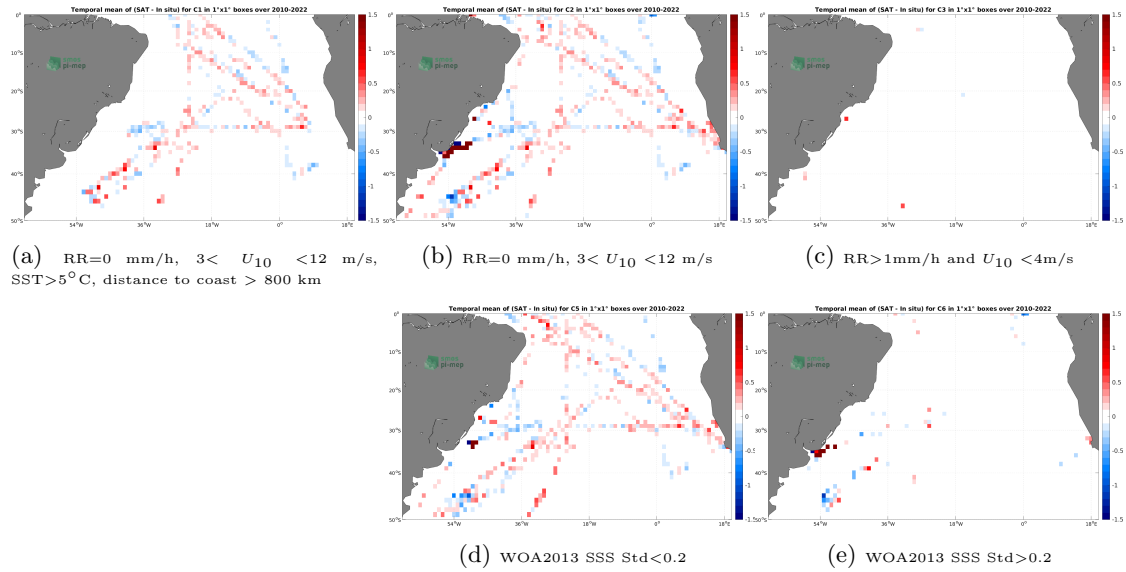
Figure 12: Temporal mean gridded over spatial boxes of size 1^\circ \times 1^\circ of \Delta SSS (SMOS SSS L3 v8 - 9 Days (CATDS-CECOS-LOCEAN) - TSG (SAMOS)) for 5 different subdatasets corresponding to:RR=0 mm/h, 3 < U_{10} < 12 m/s, SST >5^\circ\text{C} , distance to coast > 800 km (a), RR=0 mm/h, 3 < U_{10} < 12 m/s (b), RR >1 mm/h and U_{10} < 4 m/s (c), WOA2013 SSS Std <0.2 (d), WOA2013 SSS Std >0.2 (e).
