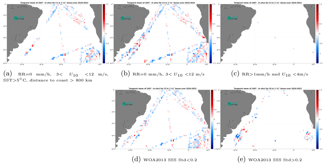
Figure 12: Temporal mean gridded over spatial boxes of size 1^\circ \times 1^\circ of \Delta SSS (SMOS SSS L3 v8 - 9 Days (CATDS-CEC-LOCEAN) - TSG (Polarstern)) for 5 different subdatasets corresponding to:RR=0 mm/h, 3 < U_{10} < 12 m/s, SST >5^\circ C, distance to coast > 800 km (a), RR=0 mm/h, 3 < U_{10} < 12 m/s (b), RR >1 mm/h and U_{10} < 4 m/s (c), WOA2013 SSS Std <0.2 (d), WOA2013 SSS Std >0.2 (e).
