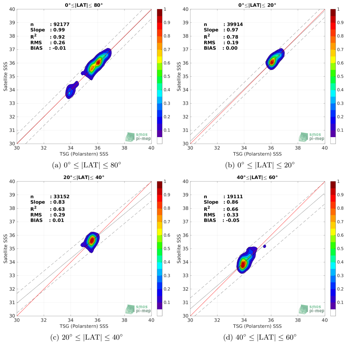
Figure 9: Contour maps of the concentration of SMOS SSS L3 v8 - 9 Days (CATDS-CECOS-LOCEAN) SSS ( y -axis) versus TSG (Polarstern) SSS ( x -axis) at match-up pairs for different latitude bands. For each plot, the red line shows x=y . The black thin and dashed lines indicate a linear fit through the data cloud and the \pm 95\% confidence levels, respectively. The number match-up pairs n , the slope and R^2 coefficient of the linear fit, the root mean square (RMS) and the mean bias between satellite and in situ data are indicated for each latitude band in each plots.
