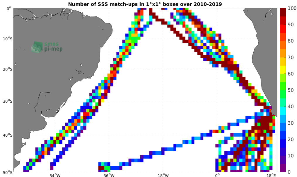
Figure 4: Number of SSS match-ups between TSG (Polarstern) SSS and the SMOS SSS L3 v8 - 9 Days (CATDS-CECOS-LOCEAN) SSS product for the South Atlantic Ocean Pi-MEP region over 1^\circ \times 1^\circ boxes and for the full satellite product period.
