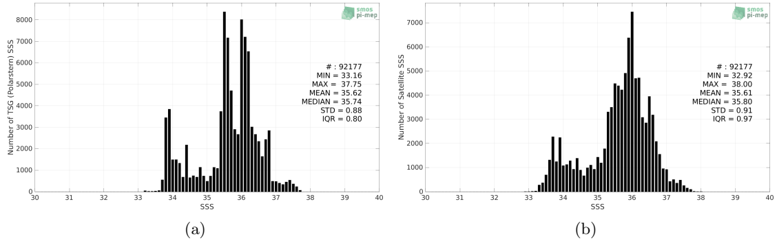
Figure 2: Histograms of SSS from TSG (Polarstern) (a) and SMOS SSS L3 v8 - 9 Days (CATDS-CECOS-LOCEAN) (b) considering all match-up pairs per bins of 0.1 over the South Atlantic Ocean Pi-MEP region and for the full satellite product period.
