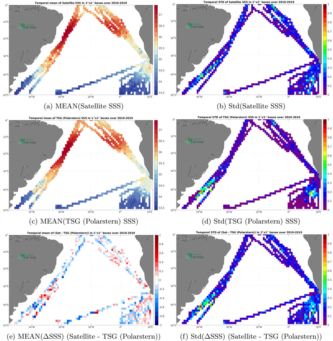
Figure 6: Temporal mean (left) and Std (right) of SSS from SMOS SSS L3 v8 - 9 Days (CATDS-CECOS-LOCEAN) (top), TSG (Polarstern) (middle), and of \Delta SSS (Satellite - TSG (Polarstern)). Only match-up pairs are used to generate these maps.
