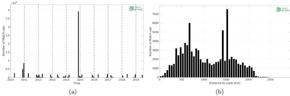
Figure 1: Number of match-ups between TSG (Polarstern) and SMOS SSS L3 v8 - 9 Days (CATDS-CECOS-LOCEAN) SSS as a function of time (a) and as function of the distance to coast (b) over the South Atlantic Ocean Pi-MEP region and for the full satellite product period.
