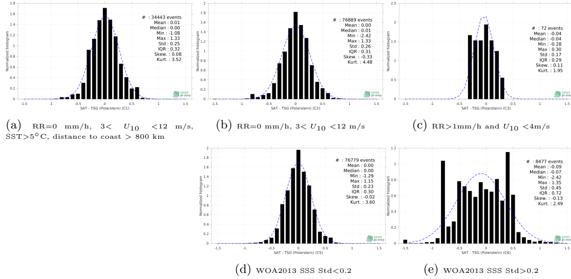
Figure 13: Normalized histogram of \Delta SSS (SMOS SSS L3 v8 - 9 Days (CATDS-CECOS-LOCEAN) - TSG (Polarstern)) for 5 different subdatasets corresponding to: RR=0 mm/h, 3 < U_{10} < 12 m/s, SST > 5°C, distance to coast > 800 km (a), RR=0 mm/h, 3 < U_{10} < 12 m/s (b), RR > 1mm/h and U_{10} < 4 m/s (c), WOA2013 SSS Std < 0.2 (d), WOA2013 SSS Std > 0.2 (e).
