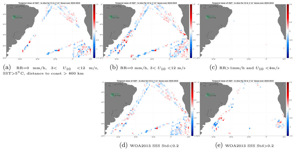
Figure 12: Temporal mean gridded over spatial boxes of size 1^\circ \times 1^\circ of \Delta\text{SSS} (SMOS SSS L3 v8 - 9 Days (CATDS-CECOS-LOCEAN) - TSG (Polarstern)) for 5 different subdatasets corresponding to:RR=0 mm/h, 3 < U_{10} < 12 m/s, SST >5^\circ\text{C} , distance to coast > 800 km (a), RR=0 mm/h, 3 < U_{10} < 12 m/s (b), RR >1 mm/h and U_{10} < 4 m/s (c), WOA2013 SSS Std <0.2 (d), WOA2013 SSS Std >0.2 (e).
