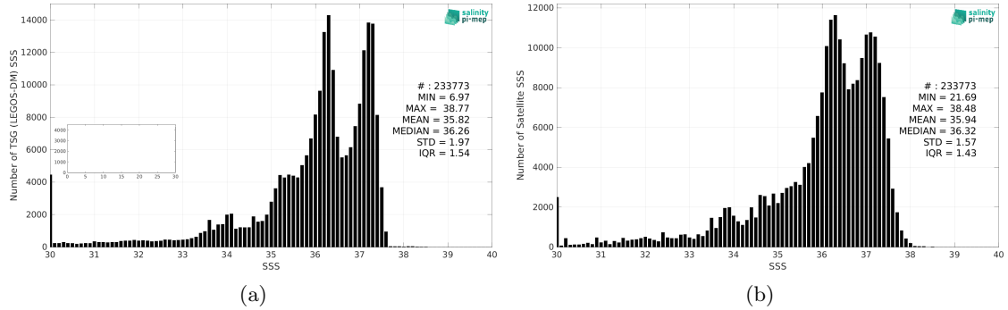
Figure 2: Histograms of SSS from TSG (LEGOS-DM) (a) and SMOS SSS L3 v8 - 9 Days (CATDS-CEC-LOCEAN) (b) considering all match-up pairs per bins of 0.1 over the South Atlantic Ocean Pi-MEP region and for the full satellite product period.
