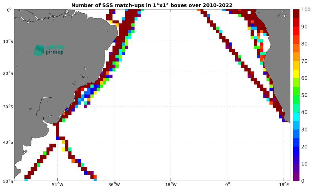
Figure 4: Number of SSS match-ups between TSG (LEGOS-DM) SSS and the SMOS SSS L3 v8 - 9 Days (CATDS-CEC-LOCEAN) SSS product for the South Atlantic Ocean Pi-MEP region over 1^\circ \times 1^\circ boxes and for the full satellite product period.
