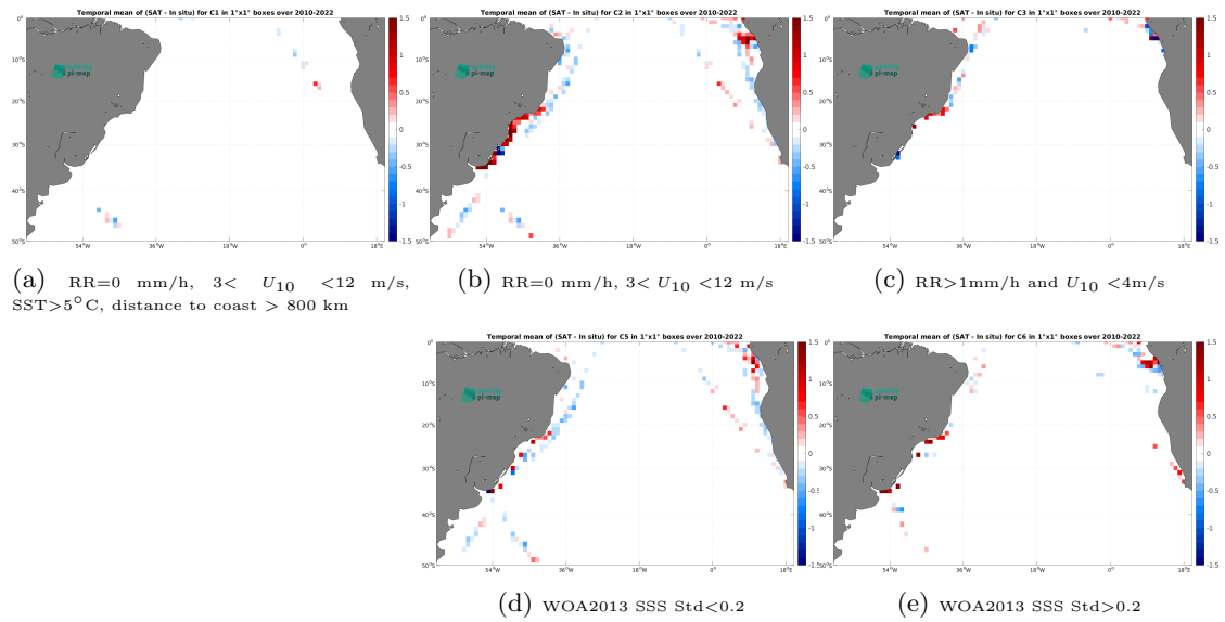
Figure 12: Temporal mean gridded over spatial boxes of size 1^\circ \times 1^\circ of \Delta SSS (SMOS SSS L3 v8 - 9 Days (CATDS-CEC-LOCEAN) - TSG (LEGOS-DM)) for 5 different subdatasets corresponding to:RR=0 mm/h, 3 < U_{10} < 12 m/s, SST >5^\circ\text{C} , distance to coast > 800 km (a), RR=0 mm/h, 3 < U_{10} < 12 m/s (b), RR >1 mm/h and U_{10} < 4 m/s (c), WOA2013 SSS Std <0.2 (d), WOA2013 SSS Std >0.2 (e).
