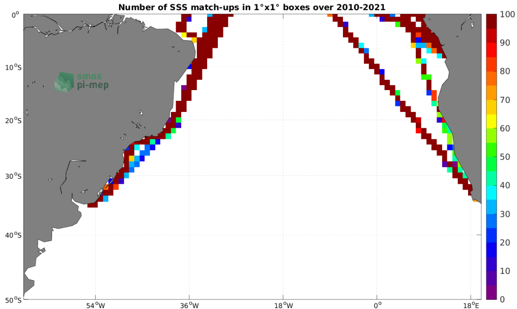
Figure 4: Number of SSS match-ups between TSG (LEGOS-DM) SSS and the SMOS SSS L3 v8 - 9 Days (CATDS-CECOS-LOCEAN) SSS product for the South Atlantic Ocean Pi-MEP region over 1^\circ \times 1^\circ boxes and for the full satellite product period.
