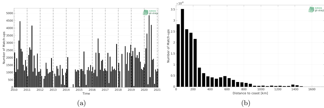
Figure 1: Number of match-ups between TSG (LEGOS-DM) and SMOS SSS L3 v8 - 9 Days (CATDS-CECOS-LOCEAN) SSS as a function of time (a) and as function of the distance to coast (b) over the South Atlantic Ocean Pi-MEP region and for the full satellite product period.
