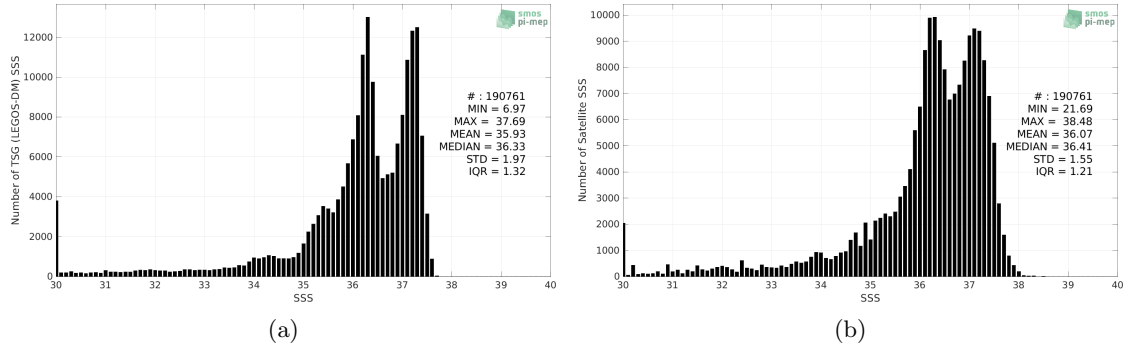
Figure 2: Histograms of SSS from TSG (LEGOS-DM) (a) and SMOS SSS L3 v8 - 9 Days (CATDS-CECOS-LOCEAN) (b) considering all match-up pairs per bins of 0.1 over the South Atlantic Ocean Pi-MEP region and for the full satellite product period.
