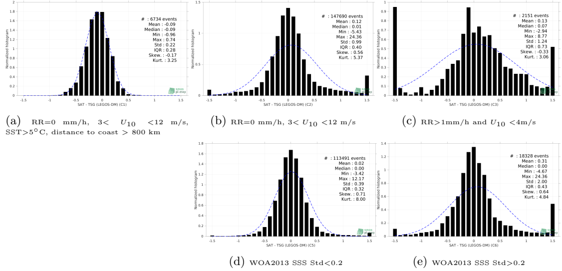
Figure 13: Normalized histogram of \Delta SSS (SMOS SSS L3 v8 - 9 Days (CATDS-CECOS-LOCEAN) - TSG (LEGOS-DM)) for 5 different subdatasets corresponding to: RR=0 mm/h, 3 < U_{10} < 12 m/s, SST > 5°C, distance to coast > 800 km (a), RR=0 mm/h, 3 < U_{10} < 12 m/s (b), RR > 1mm/h and U_{10} < 4 m/s (c), WOA2013 SSS Std < 0.2 (d), WOA2013 SSS Std > 0.2 (e).
