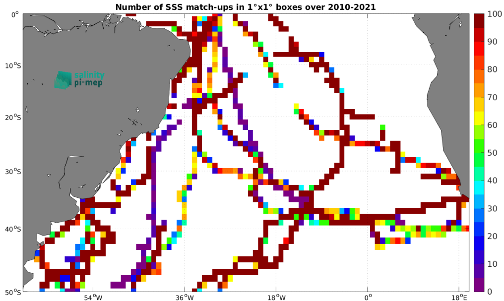
Figure 4: Number of SSS match-ups between TSG (GOSUD-Sailing-ship) SSS and the SMOS SSS L3 v8 - 9 Days (CATDS-CEC-LOCEAN) SSS product for the South Atlantic Ocean Pi-MEP region over 1^\circ \times 1^\circ boxes and for the full satellite product period.
