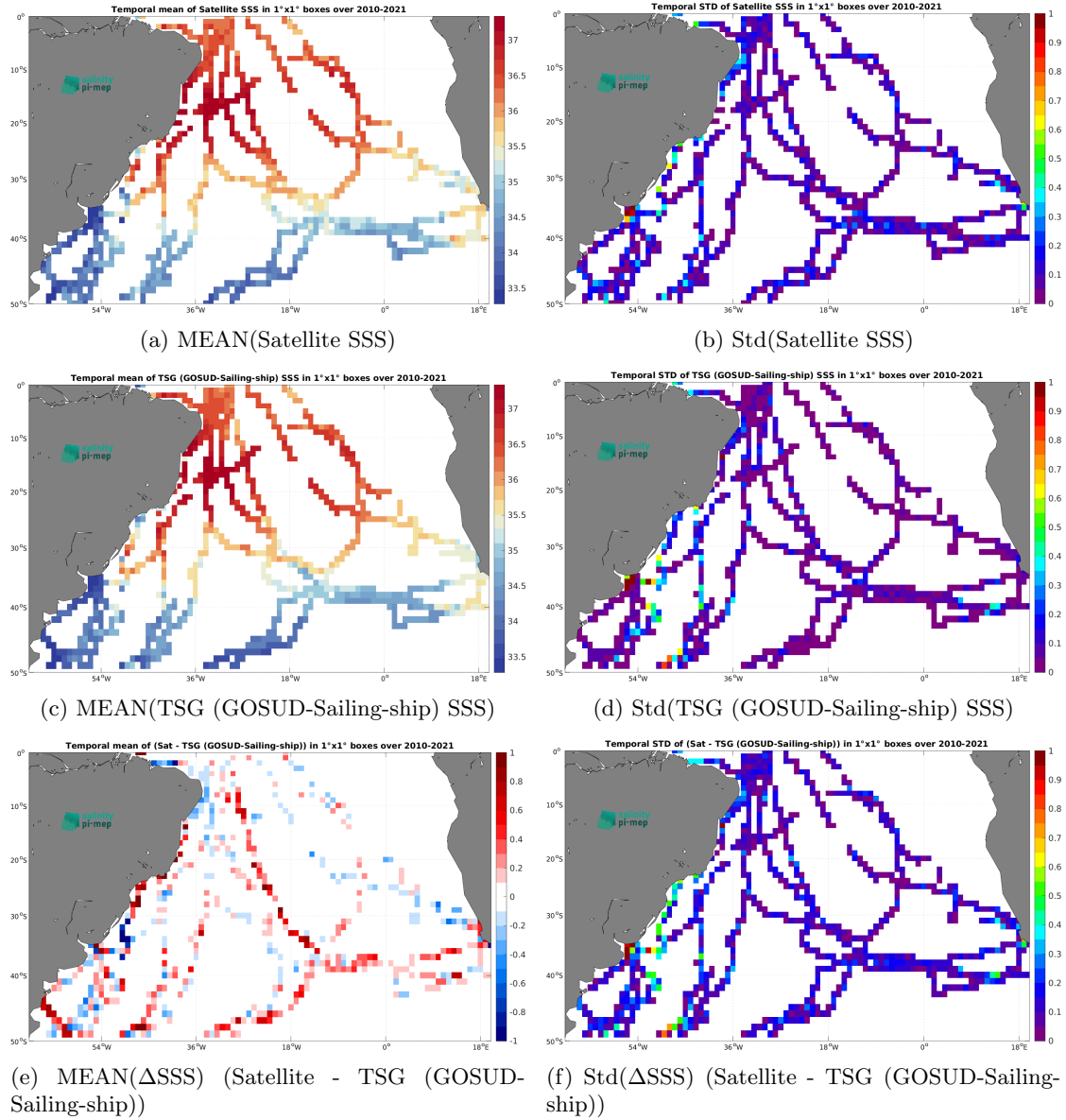
Figure 6: Temporal mean (left) and Std (right) of SSS from SMOS SSS L3 v8 - 9 Days (CATDS-CEC-LOCEAN) (top), TSG (GOSUD-Sailing-ship) (middle), and of \Delta SSS (Satellite - TSG (GOSUD-Sailing-ship)). Only match-up pairs are used to generate these maps.
