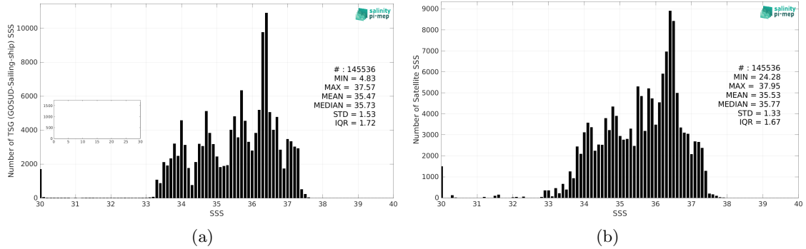
Figure 2: Histograms of SSS from TSG (GOSUD-Sailing-ship) (a) and SMOS SSS L3 v8 - 9 Days (CATDS-CEC-LOCEAN) (b) considering all match-up pairs per bins of 0.1 over the South Atlantic Ocean Pi-MEP region and for the full satellite product period.
