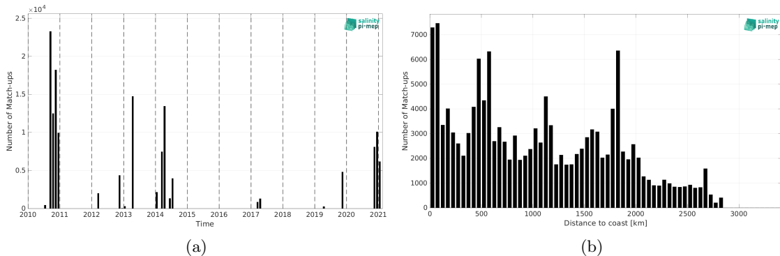
Figure 1: Number of match-ups between TSG (GOSUD-Sailing-ship) and SMOS SSS L3 v8 - 9 Days (CATDS-CEC-LOCEAN) SSS as a function of time (a) and as function of the distance to coast (b) over the South Atlantic Ocean Pi-MEP region and for the full satellite product period.
