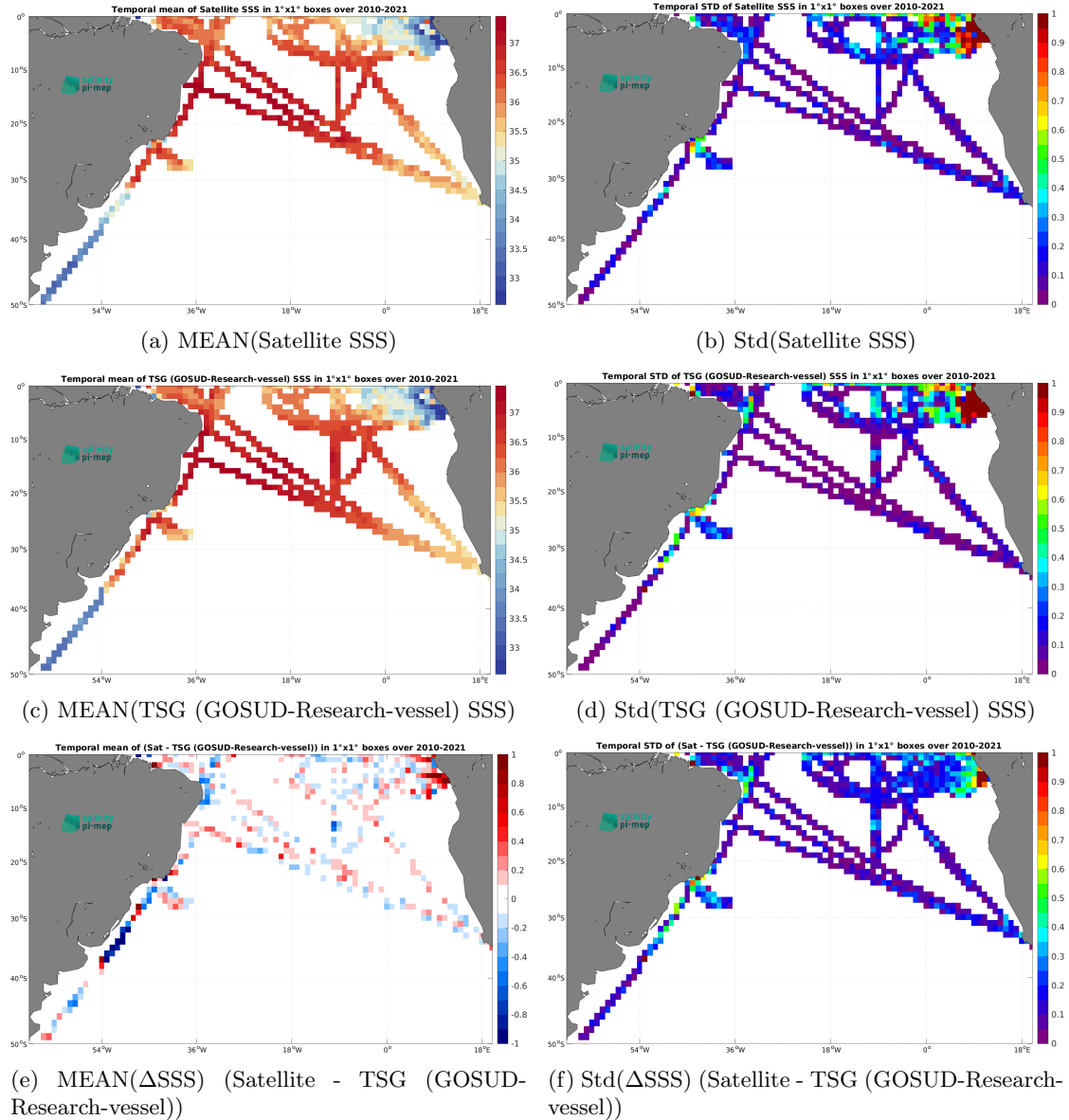
Figure 6: Temporal mean (left) and Std (right) of SSS from SMOS SSS L3 v8 - 9 Days (CATDS-CEC-LOCEAN) (top), TSG (GOSUD-Research-vessel) (middle), and of \Delta SSS (Satellite - TSG (GOSUD-Research-vessel)). Only match-up pairs are used to generate these maps.
