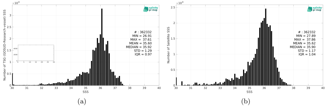
Figure 2: Histograms of SSS from TSG (GOSUD-Research-vessel) (a) and SMOS SSS L3 v8 - 9 Days (CATDS-CEC-LOCEAN) (b) considering all match-up pairs per bins of 0.1 over the South Atlantic Ocean Pi-MEP region and for the full satellite product period.
