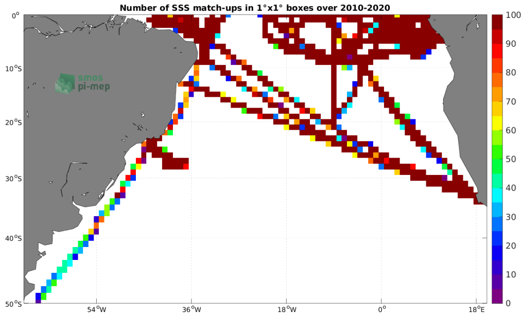
Figure 4: Number of SSS match-ups between TSG (GOSUD-Research-vessel) SSS and the SMOS SSS L3 v8 - 9 Days (CATDS-CECOS-LOCEAN) SSS product for the South Atlantic Ocean Pi-MEP region over 1^\circ \times 1^\circ boxes and for the full satellite product period.
