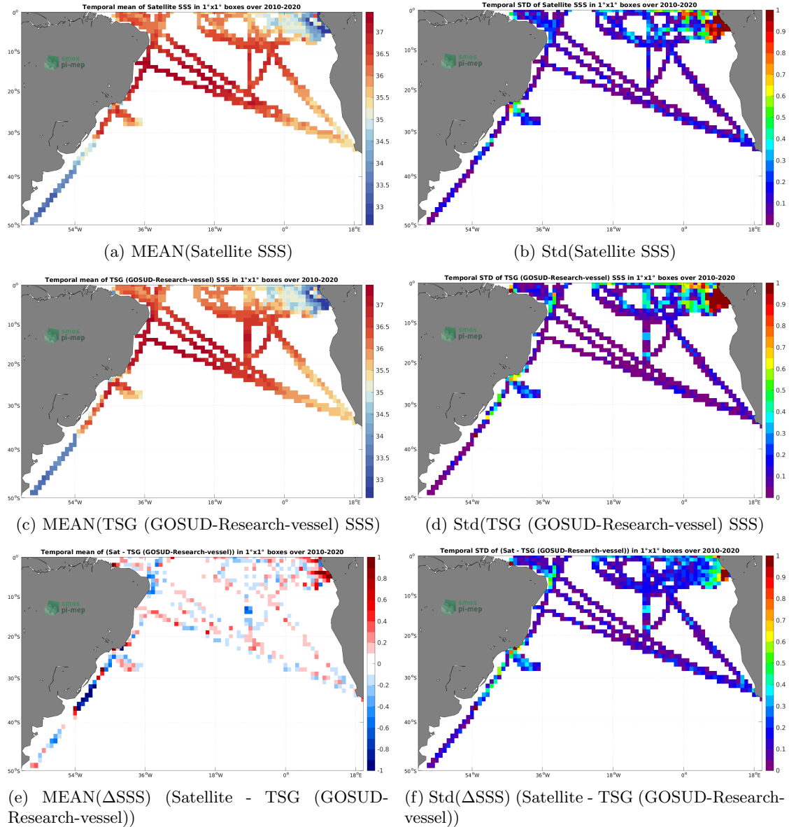
Figure 6: Temporal mean (left) and Std (right) of SSS from SMOS SSS L3 v8 - 9 Days (CATDS-CECOS-LOCEAN) (top), TSG (GOSUD-Research-vessel) (middle), and of \Delta SSS (Satellite - TSG (GOSUD-Research-vessel)). Only match-up pairs are used to generate these maps.
