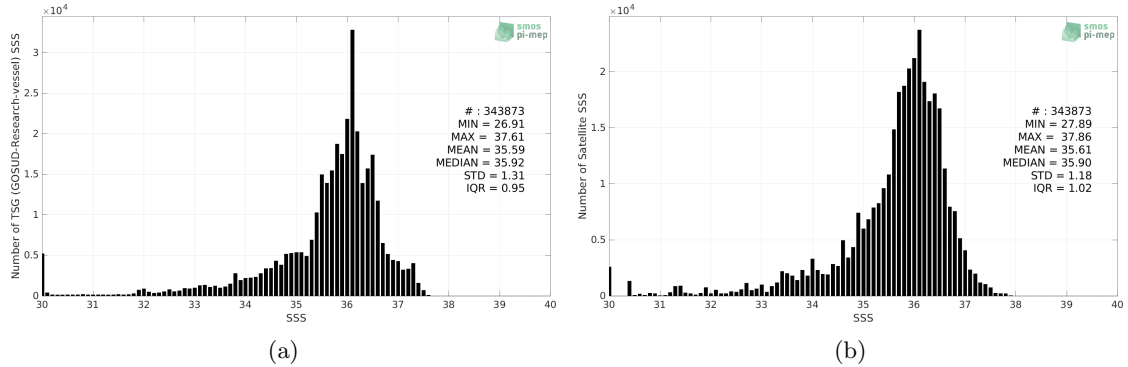
Figure 2: Histograms of SSS from TSG (GOSUD-Research-vessel) (a) and SMOS SSS L3 v8 - 9 Days (CATDS-CECOS-LOCEAN) (b) considering all match-up pairs per bins of 0.1 over the South Atlantic Ocean Pi-MEP region and for the full satellite product period.
