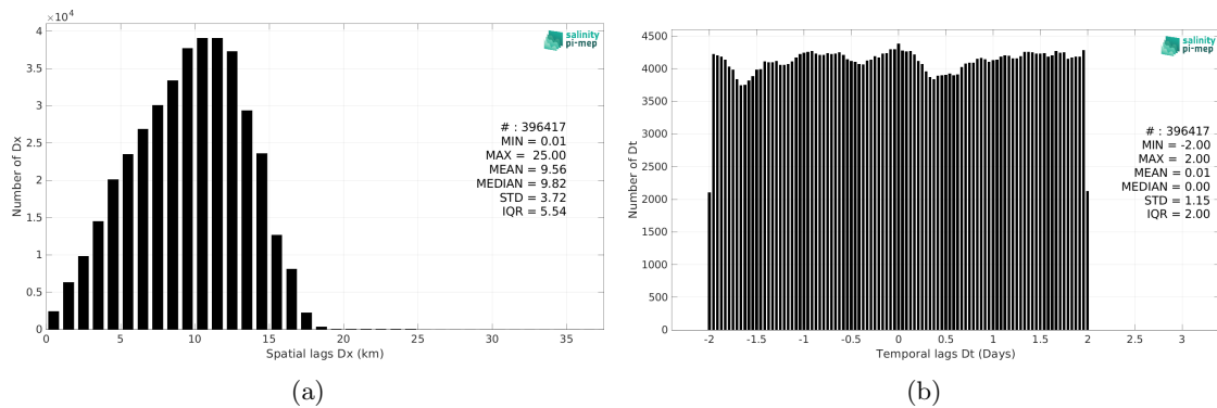
Figure 5: Histograms of the spatial (a) and temporal (b) lags between the location/time of the TSG (CSIC-UTM) measurement and the date of the corresponding SMOS SSS L3 v8 - 9 Days (CATDS-CEC-LOCEAN) SSS pixel.
