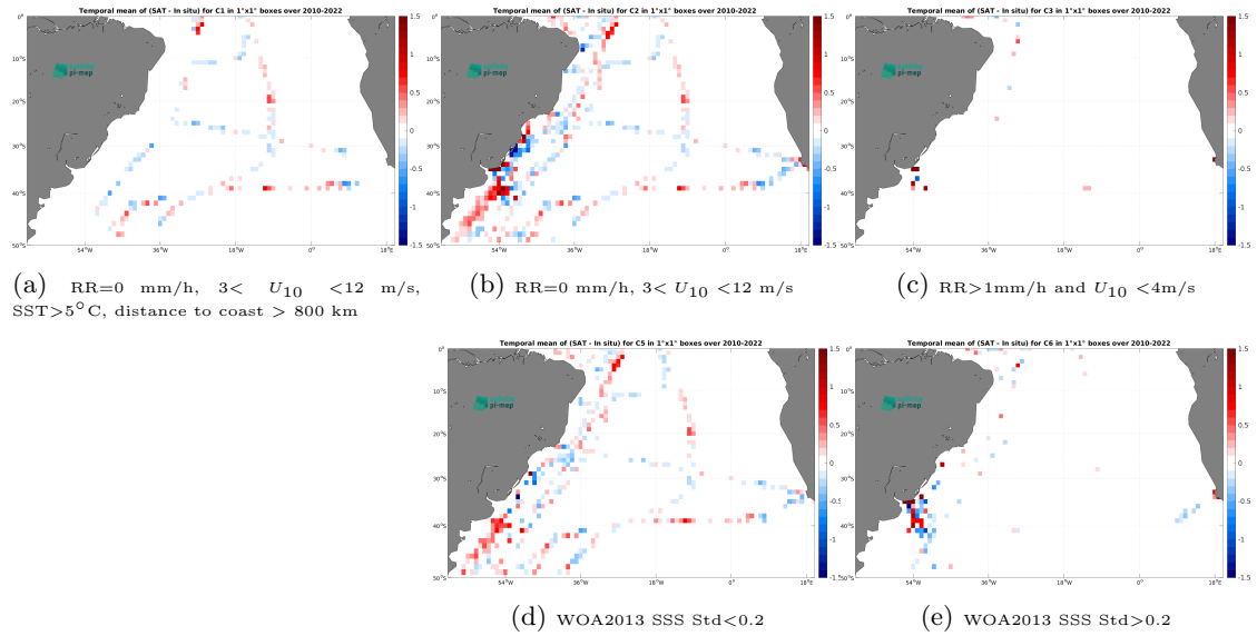
Figure 12: Temporal mean gridded over spatial boxes of size 1^\circ \times 1^\circ of \Delta SSS (SMOS SSS L3 v8 - 9 Days (CATDS-CEC-LOCEAN) - TSG (CSIC-UTM)) for 5 different subdatasets corresponding to:RR=0 mm/h, 3 < U_{10} < 12 m/s, SST >5^\circ C, distance to coast > 800 km (a), RR=0 mm/h, 3 < U_{10} < 12 m/s (b), RR >1 mm/h and U_{10} < 4 m/s (c), WOA2013 SSS Std <0.2 (d), WOA2013 SSS Std >0.2 (e).
