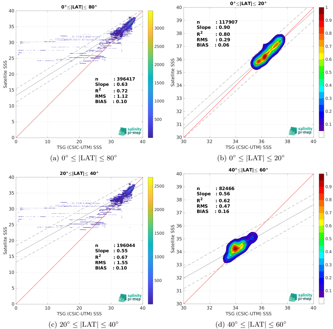
Figure 9: Contour maps of the concentration of SMOS SSS L3 v8 - 9 Days (CATDS-CEC-LOCEAN) SSS (y-axis) versus TSG (CSIC-UTM) SSS (x-axis) at match-up pairs for different latitude bands. For each plot, the red line shows x=y . The black thin and dashed lines indicate a linear fit through the data cloud and the \pm 95\% confidence levels, respectively. The number of match-up pairs n , the slope and R^2 coefficient of the linear fit, the root mean square (RMS) and the mean bias between satellite and in situ data are indicated for each latitude band in each plot.
