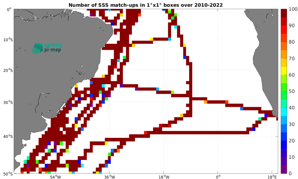
Figure 4: Number of SSS match-ups between TSG (CSIC-UTM) SSS and the SMOS SSS L3 v8 - 9 Days (CATDS-CEC-LOCEAN) SSS product for the South Atlantic Ocean Pi-MEP region over 1^\circ \times 1^\circ boxes and for the full satellite product period.
