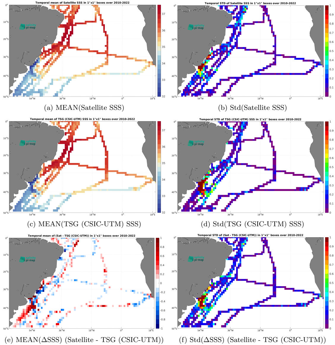
Figure 6: Temporal mean (left) and Std (right) of SSS from SMOS SSS L3 v8 - 9 Days (CATDS-CEC-LOCEAN) (top), TSG (CSIC-UTM) (middle), and of \Delta SSS (Satellite - TSG (CSIC-UTM)). Only match-up pairs are used to generate these maps.
