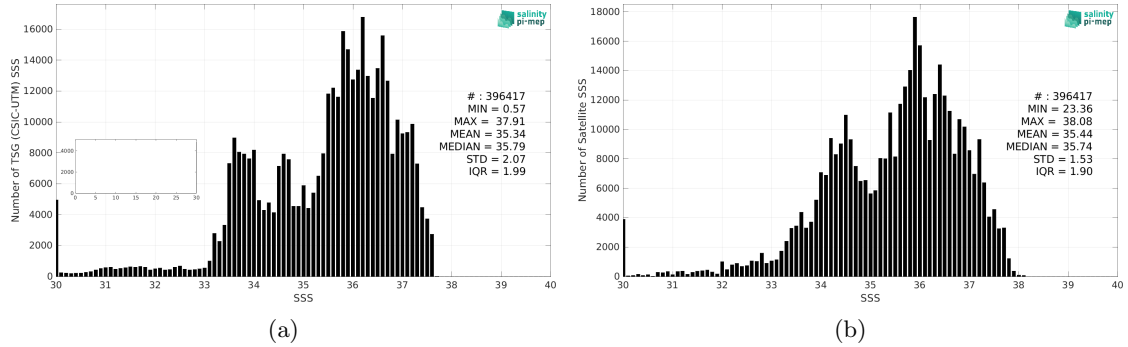
Figure 2: Histograms of SSS from TSG (CSIC-UTM) (a) and SMOS SSS L3 v8 - 9 Days (CATDS-CEC-LOCEAN) (b) considering all match-up pairs per bins of 0.1 over the South Atlantic Ocean Pi-MEP region and for the full satellite product period.
