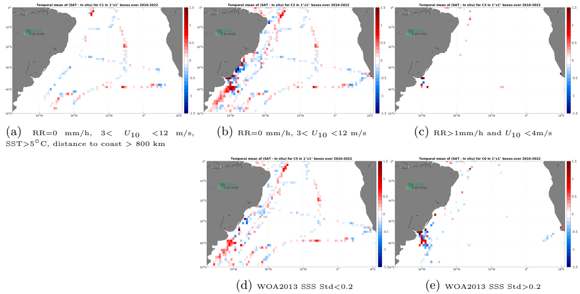
Figure 12: Temporal mean gridded over spatial boxes of size 1^\circ \times 1^\circ of \Delta SSS (SMOS SSS L3 v8 - 9 Days (CATDS-CECOS-LOCEAN) - TSG (CSIC-UTM)) for 5 different subdatasets corresponding to:RR=0 mm/h, 3 < U_{10} < 12 m/s, SST >5^\circ\text{C} , distance to coast > 800 km (a), RR=0 mm/h, 3 < U_{10} < 12 m/s (b), RR >1 mm/h and U_{10} < 4 m/s (c), WOA2013 SSS Std <0.2 (d), WOA2013 SSS Std >0.2 (e).
