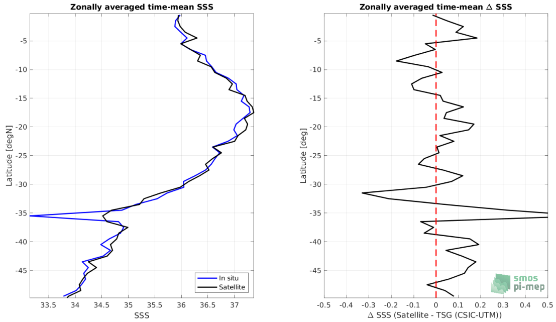
Figure 8: Left panel: Zonal mean SSS from SMOS SSS L3 v8 - 9 Days (CATDS-CECOS-LOCEAN) satellite product (black) and from TSG (CSIC-UTM) (blue). Right panel: Zonal mean of \Delta SSS (Satellite - TSG (CSIC-UTM)) for all the collected Pi-MEP match-up pairs estimated over the full satellite product period.
