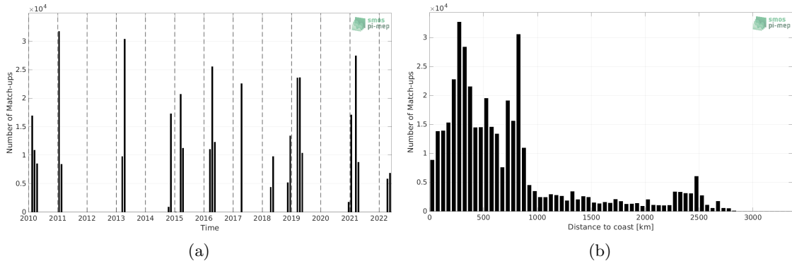
Figure 1: Number of match-ups between TSG (CSIC-UTM) and SMOS SSS L3 v8 - 9 Days (CATDS-CECOS-LOCEAN) SSS as a function of time (a) and as function of the distance to coast (b) over the South Atlantic Ocean Pi-MEP region and for the full satellite product period.
