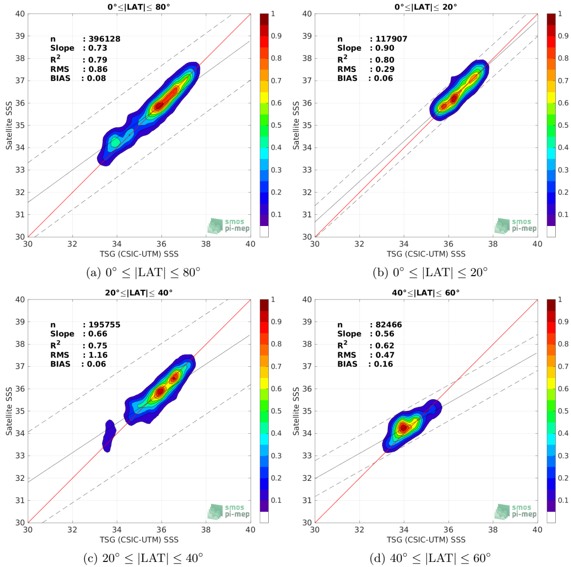
Figure 9: Contour maps of the concentration of SMOS SSS L3 v8 - 9 Days (CATDS-CECOS-LOCEAN) SSS ( y -axis) versus TSG (CSIC-UTM) SSS ( x -axis) at match-up pairs for different latitude bands. For each plot, the red line shows x=y . The black thin and dashed lines indicate a linear fit through the data cloud and the \pm 95\% confidence levels, respectively. The number match-up pairs n , the slope and R^2 coefficient of the linear fit, the root mean square (RMS) and the mean bias between satellite and in situ data are indicated for each latitude band in each plots.
