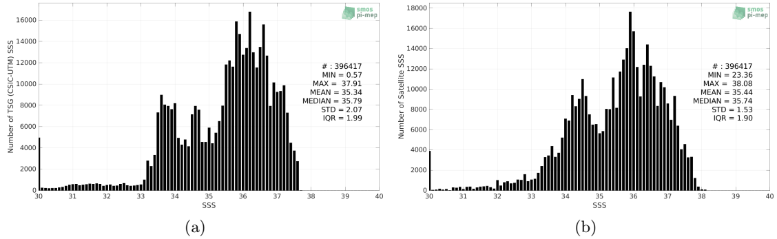
Figure 2: Histograms of SSS from TSG (CSIC-UTM) (a) and SMOS SSS L3 v8 - 9 Days (CATDS-CECOS-LOCEAN) (b) considering all match-up pairs per bins of 0.1 over the South Atlantic Ocean Pi-MEP region and for the full satellite product period.
