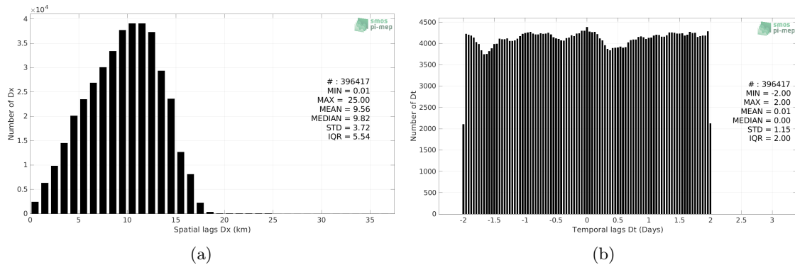
Figure 5: Histograms of the spatial (a) and temporal (b) lags between the location/time of the TSG (CSIC-UTM) measurement and the date of the corresponding SMOS SSS L3 v8 - 9 Days (CATDS-CECOS-LOCEAN) SSS pixel.
