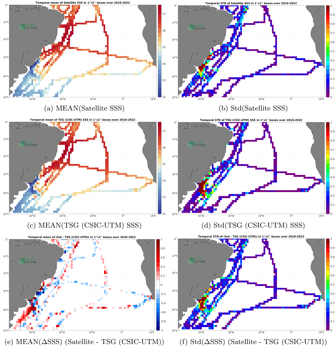
Figure 6: Temporal mean (left) and Std (right) of SSS from SMOS SSS L3 v8 - 9 Days (CATDS-CECOS-LOCEAN) (top), TSG (CSIC-UTM) (middle), and of \Delta SSS (Satellite - TSG (CSIC-UTM)). Only match-up pairs are used to generate these maps.
