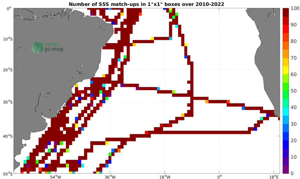
Figure 4: Number of SSS match-ups between TSG (CSIC-UTM) SSS and the SMOS SSS L3 v8 - 9 Days (CATDS-CECOS-LOCEAN) SSS product for the South Atlantic Ocean Pi-MEP region over 1^\circ \times 1^\circ boxes and for the full satellite product period.
