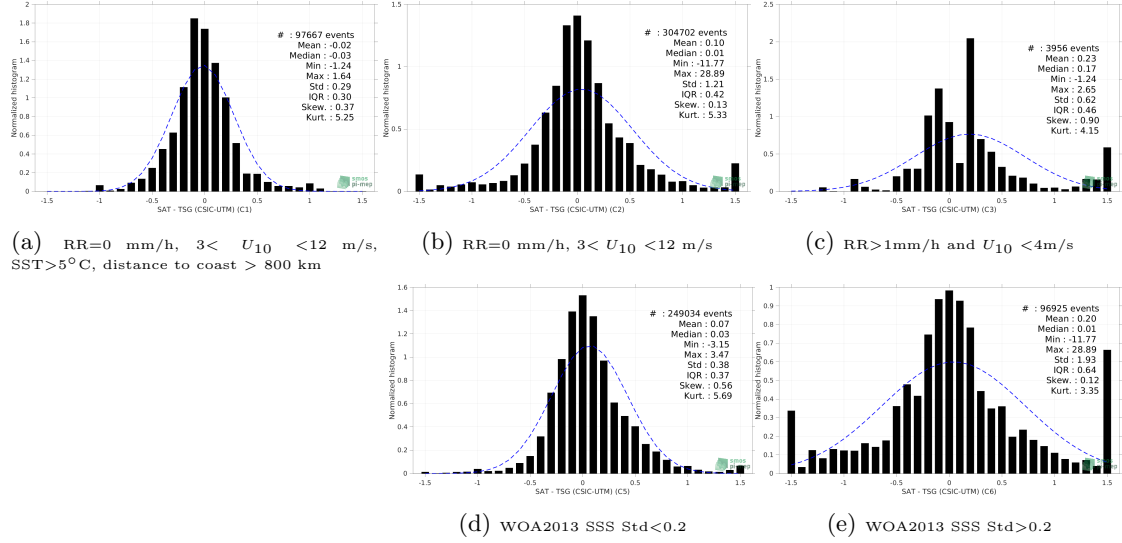
Figure 13: Normalized histogram of \Delta SSS (SMOS SSS L3 v8 - 9 Days (CATDS-CECOS-LOCEAN) - TSG (CSIC-UTM)) for 5 different subdatasets corresponding to: RR=0 mm/h, 3 < U_{10} < 12 m/s, SST > 5°C, distance to coast > 800 km (a), RR=0 mm/h, 3 < U_{10} < 12 m/s (b), RR > 1mm/h and U_{10} < 4 m/s (c), WOA2013 SSS Std < 0.2 (d), WOA2013 SSS Std > 0.2 (e).
