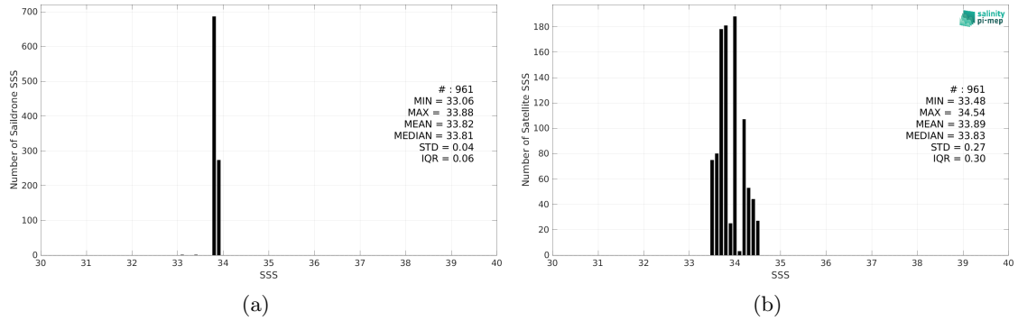
Figure 2: Histograms of SSS from Saildrone (a) and SMOS SSS L3 v8 - 9 Days (CATDS-CEC-LOCEAN) (b) considering all match-up pairs per bins of 0.1 over the South Atlantic Ocean Pi-MEP region and for the full satellite product period.
