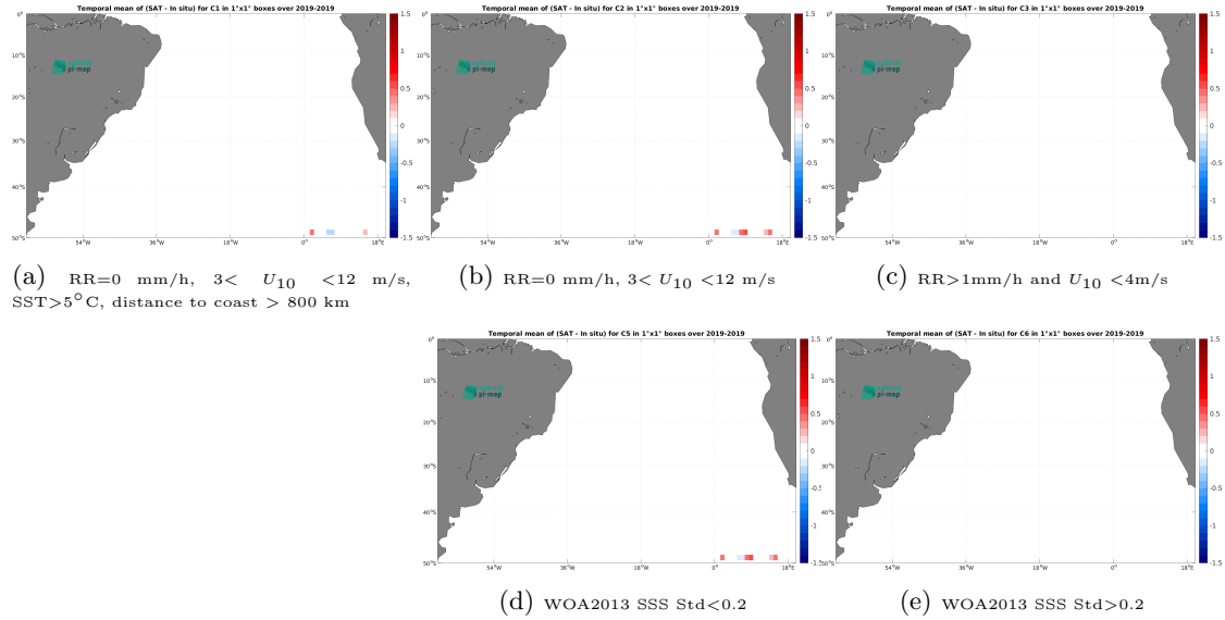
Figure 12: Temporal mean gridded over spatial boxes of size 1^{\circ}\times 1^{\circ} of \Delta\text{SSS} (SMOS SSS L3 v8 - 9 Days (CATDS-CEC-LOCEAN) - Saildrone) for 5 different subdatasets corresponding to:RR=0 mm/h, 3 < U_{10} < 12 m/s, SST >5^{\circ}\text{C} , distance to coast > 800 km (a), RR=0 mm/h, 3 < U_{10} < 12 m/s (b), RR >1 mm/h and U_{10} < 4 m/s (c), WOA2013 SSS Std <0.2 (d), WOA2013 SSS Std >0.2 (e).
