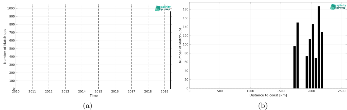
Figure 1: Number of match-ups between Saildrone and SMOS SSS L3 v8 - 9 Days (CATDS-CEC-LOCEAN) SSS as a function of time (a) and as function of the distance to coast (b) over the South Atlantic Ocean Pi-MEP region and for the full satellite product period.
