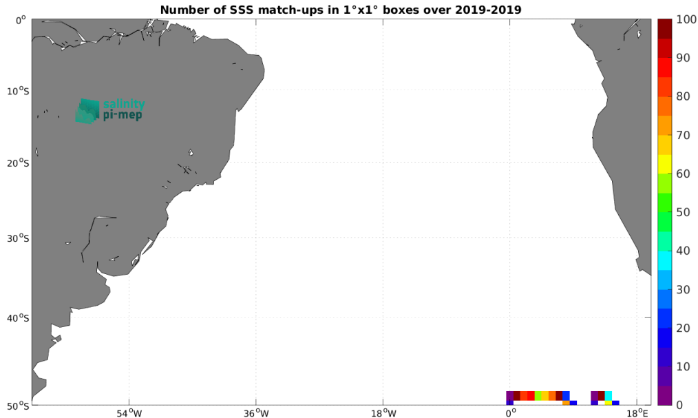
Figure 4: Number of SSS match-ups between Saildrone SSS and the SMOS SSS L3 v8 - 9 Days (CATDS-CEC-LOCEAN) SSS product for the South Atlantic Ocean Pi-MEP region over 1^\circ \times 1^\circ boxes and for the full satellite product period.
