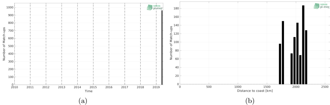
Figure 1: Number of match-ups between Saildrone and SMOS SSS L3 v8 - 9 Days (CATDS-CECOS-LOCEAN) SSS as a function of time (a) and as function of the distance to coast (b) over the South Atlantic Ocean Pi-MEP region and for the full satellite product period.
