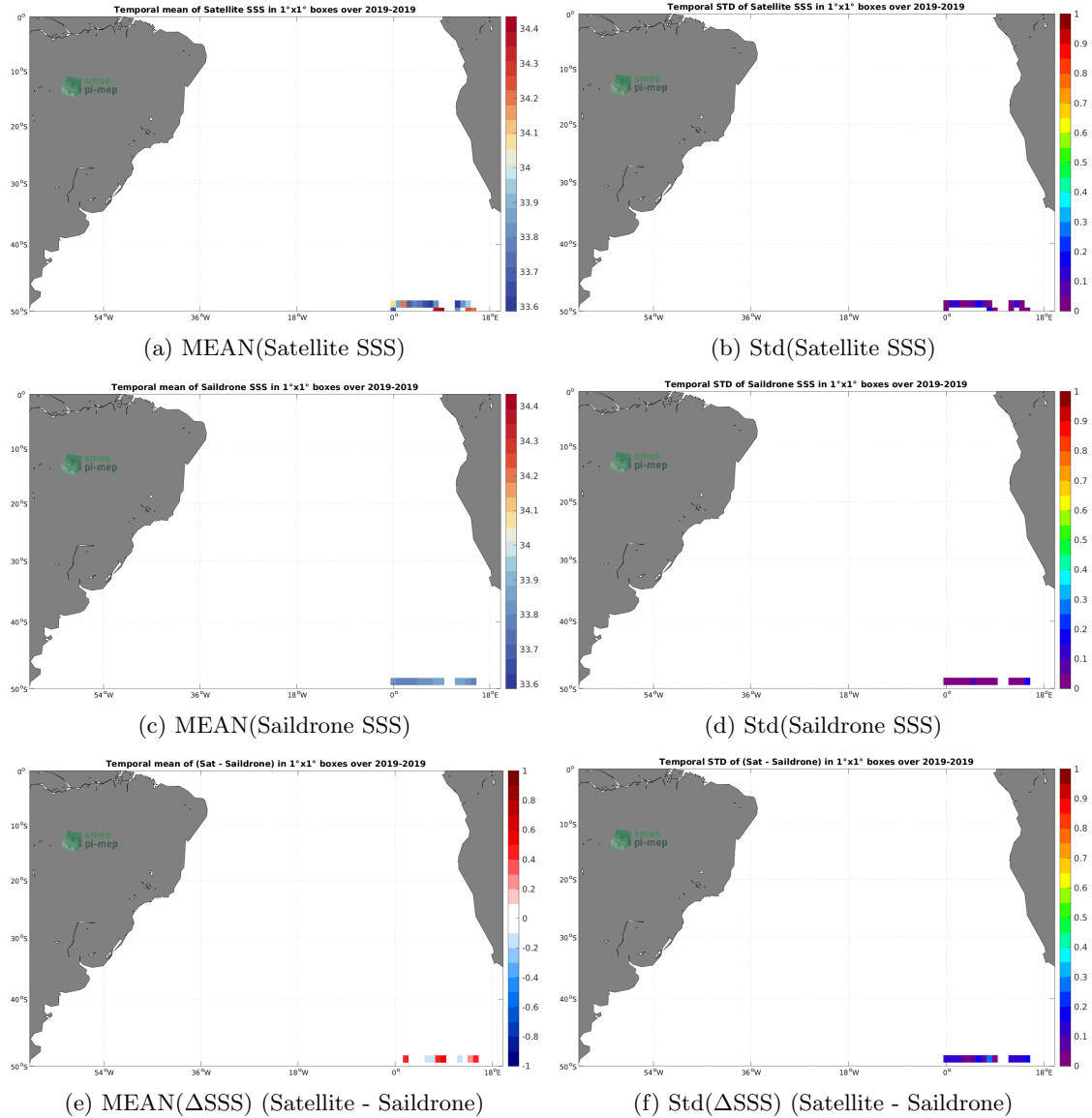
Figure 6: Temporal mean (left) and Std (right) of SSS from SMOS SSS L3 v8 - 9 Days (CATDS-CECOS-LOCEAN) (top), Saildrone (middle), and of \Delta SSS (Satellite - Saildrone). Only match-up pairs are used to generate these maps.
