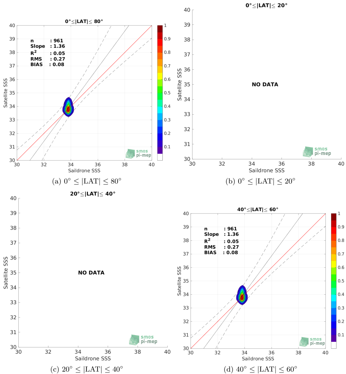
Figure 9: Contour maps of the concentration of SMOS SSS L3 v8 - 9 Days (CATDS-CECOS-LOCEAN) SSS (y-axis) versus Saildrone SSS (x-axis) at match-up pairs for different latitude bands. For each plot, the red line shows x=y . The black thin and dashed lines indicate a linear fit through the data cloud and the \pm 95\% confidence levels, respectively. The number match-up pairs n , the slope and R^2 coefficient of the linear fit, the root mean square (RMS) and the mean bias between satellite and in situ data are indicated for each latitude band in each plots.
