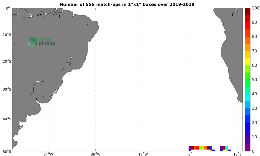
Figure 4: Number of SSS match-ups between Saildrone SSS and the SMOS SSS L3 v8 - 9 Days (CATDS-CECOS-LOCEAN) SSS product for the South Atlantic Ocean Pi-MEP region over 1^\circ \times 1^\circ boxes and for the full satellite product period.
