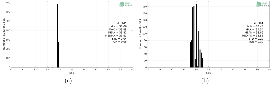
Figure 2: Histograms of SSS from Saildrone (a) and SMOS SSS L3 v8 - 9 Days (CATDS-CECOS-LOCEAN) (b) considering all match-up pairs per bins of 0.1 over the South Atlantic Ocean Pi-MEP region and for the full satellite product period.
