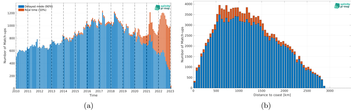
Figure 1: Number of match-ups between Argo and SMOS SSS L3 v8 - 9 Days (CATDS-CEC-LOCEAN) SSS as a function of time (a) and as function of the distance to coast (b) over the South Atlantic Ocean Pi-MEP region and for the full satellite product period.
