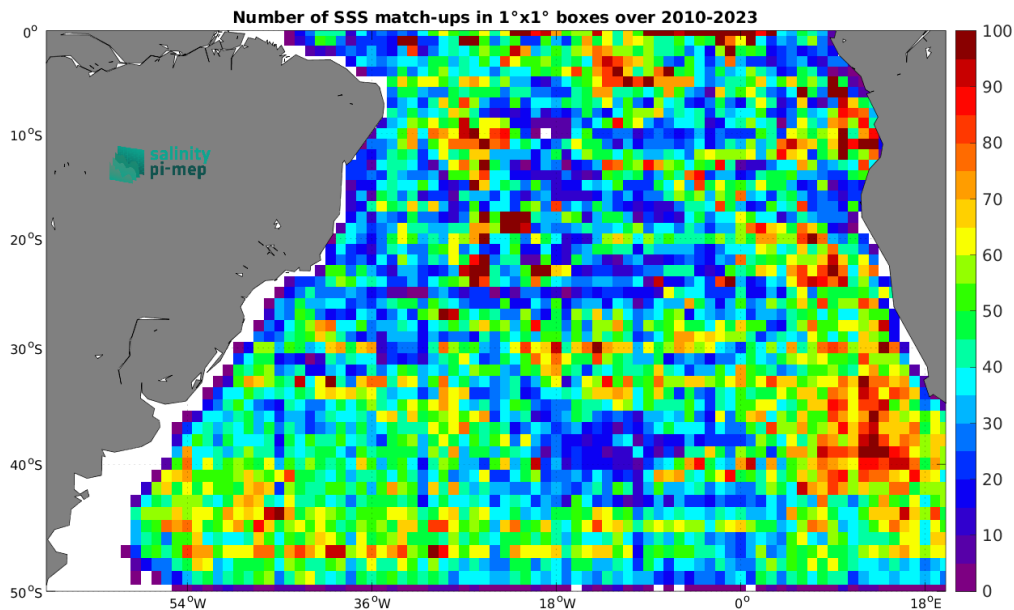
Figure 4: Number of SSS match-ups between Argo SSS and the SMOS SSS L3 v8 - 9 Days (CATDS-CEC-LOCEAN) SSS product for the South Atlantic Ocean Pi-MEP region over 1^\circ \times 1^\circ boxes and for the full satellite product period.
