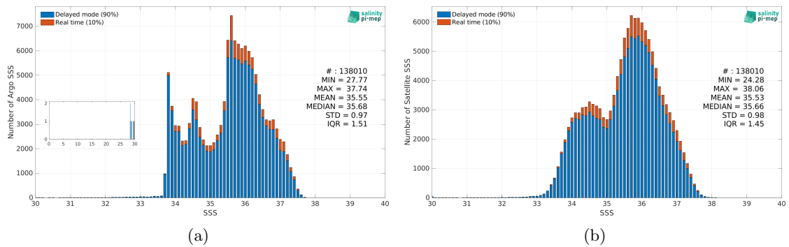
Figure 2: Histograms of SSS from Argo (a) and SMOS SSS L3 v8 - 9 Days (CATDS-CEC-LOCEAN) (b) considering all match-up pairs per bins of 0.1 over the South Atlantic Ocean Pi-MEP region and for the full satellite product period.
