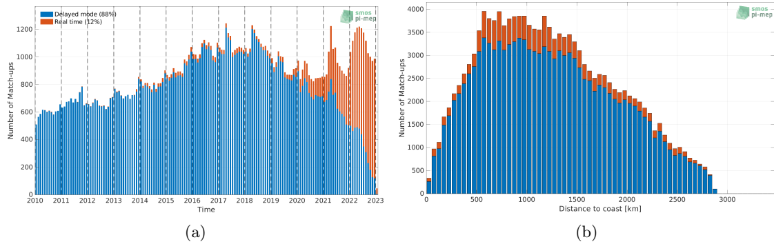
Figure 1: Number of match-ups between Argo and SMOS SSS L3 v8 - 9 Days (CATDS-CECOS-LOCEAN) SSS as a function of time (a) and as function of the distance to coast (b) over the South Atlantic Ocean Pi-MEP region and for the full satellite product period.
