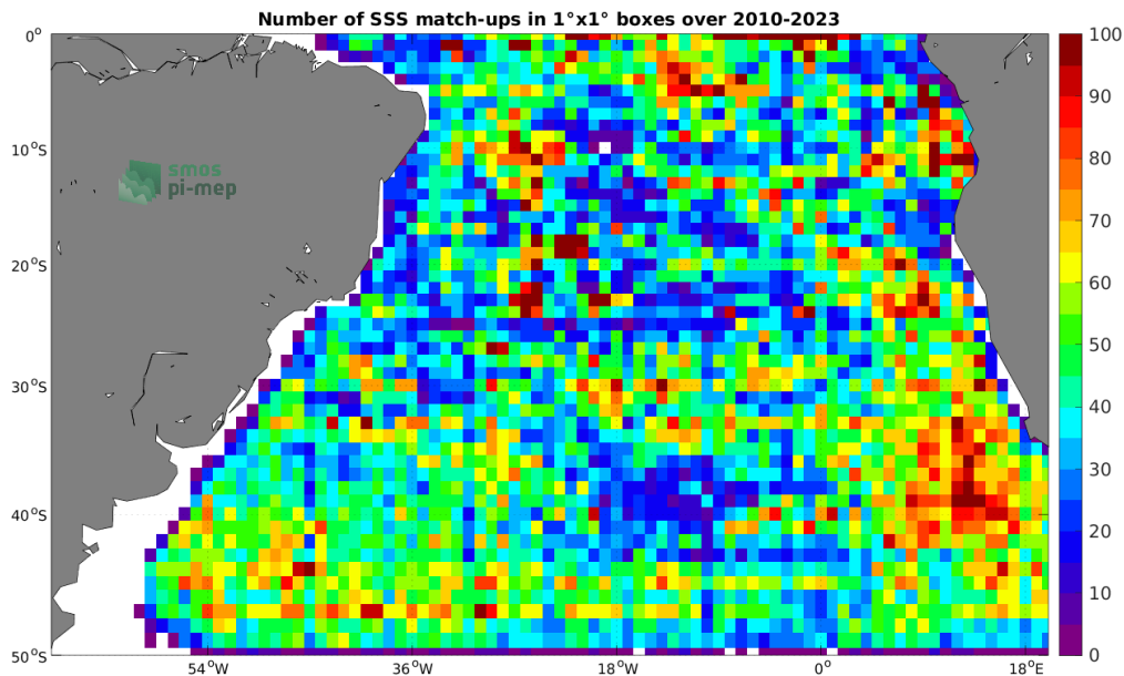
Figure 4: Number of SSS match-ups between Argo SSS and the SMOS SSS L3 v8 - 9 Days (CATDS-CECOS-LOCEAN) SSS product for the South Atlantic Ocean Pi-MEP region over 1^\circ \times 1^\circ boxes and for the full satellite product period.
