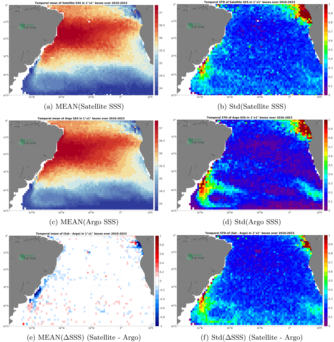
Figure 6: Temporal mean (left) and Std (right) of SSS from SMOS SSS L3 v8 - 9 Days (CATDS-CECOS-LOCEAN) (top), Argo (middle), and of \Delta SSS (Satellite - Argo). Only match-up pairs are used to generate these maps.
