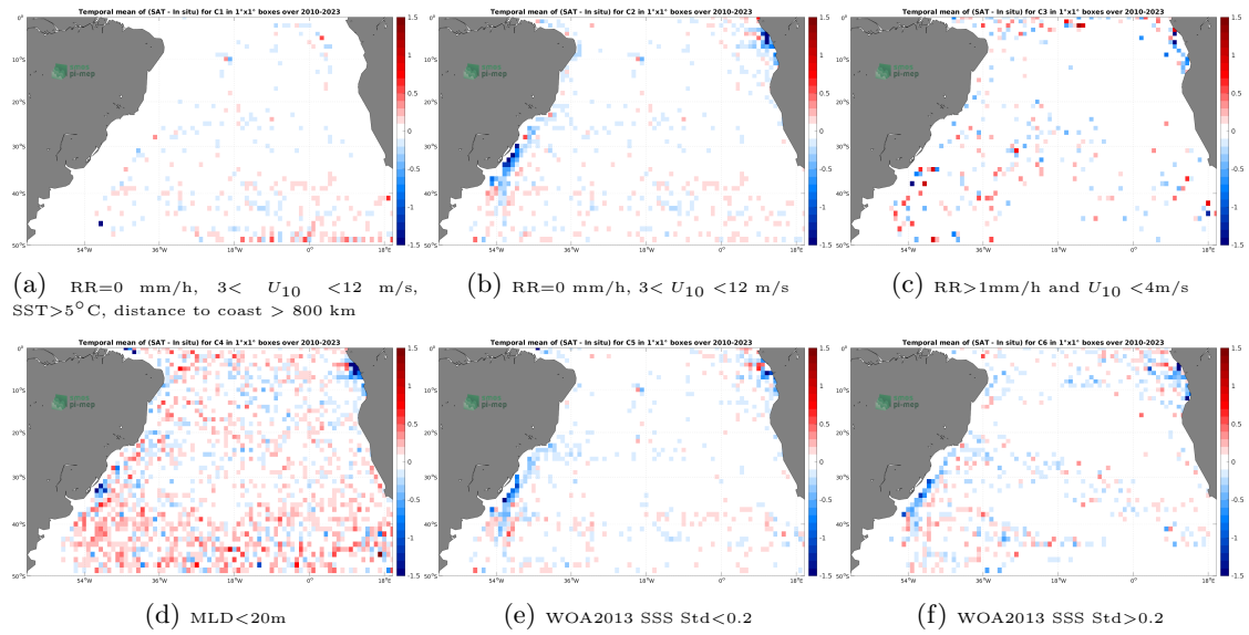
Figure 12: Temporal mean gridded over spatial boxes of size 1^\circ \times 1^\circ of \Delta SSS (SMOS SSS L3 v8 - 9 Days (CATDS-CECOS-LOCEAN) - Argo) for 6 different subdatasets corresponding to:RR=0 mm/h, 3 < U_{10} < 12 m/s, SST > 5^\circ\text{C} , distance to coast > 800 km (a), RR=0 mm/h, 3 < U_{10} < 12 m/s (b), RR > 1 mm/h and U_{10} < 4 m/s (c),MLD < 20 m (d),WOA2013 SSS Std < 0.2 (e),WOA2013 SSS Std > 0.2 (f).
