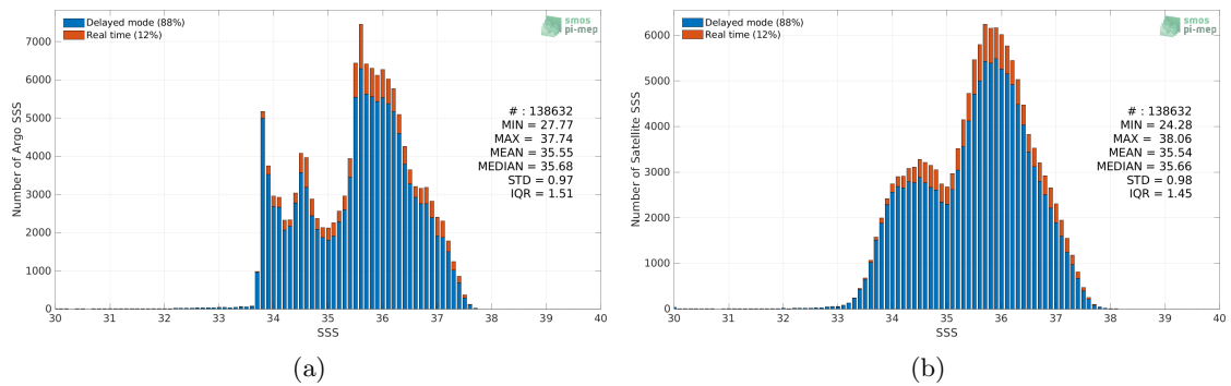
Figure 2: Histograms of SSS from Argo (a) and SMOS SSS L3 v8 - 9 Days (CATDS-CECOS-LOCEAN) (b) considering all match-up pairs per bins of 0.1 over the South Atlantic Ocean Pi-MEP region and for the full satellite product period.
