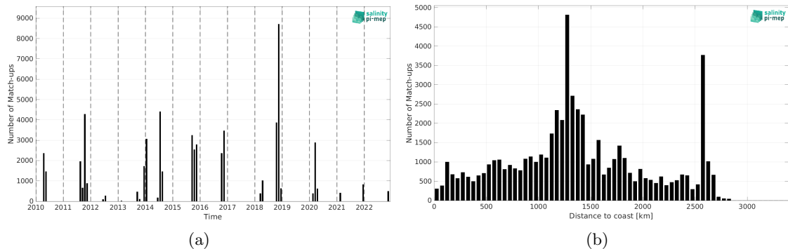
Figure 1: Number of match-ups between TSG (SAMOS) and SMOS SSS L3 v8 - 18 Days (CATDS-CEC-LOCEAN) SSS as a function of time (a) and as function of the distance to coast (b) over the South Atlantic Ocean Pi-MEP region and for the full satellite product period.
