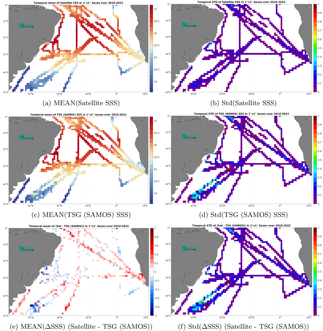
Figure 6: Temporal mean (left) and Std (right) of SSS from SMOS SSS L3 v8 - 18 Days (CATDS-CEC-LOCEAN) (top), TSG (SAMOS) (middle), and of \Delta SSS (Satellite - TSG (SAMOS)). Only match-up pairs are used to generate these maps.
