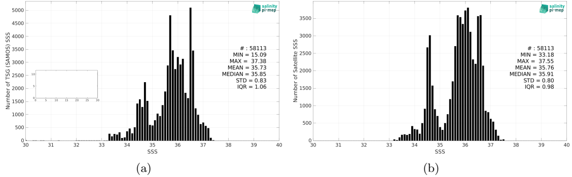
Figure 2: Histograms of SSS from TSG (SAMOS) (a) and SMOS SSS L3 v8 - 18 Days (CATDS-CEC-LOCEAN) (b) considering all match-up pairs per bins of 0.1 over the South Atlantic Ocean Pi-MEP region and for the full satellite product period.
