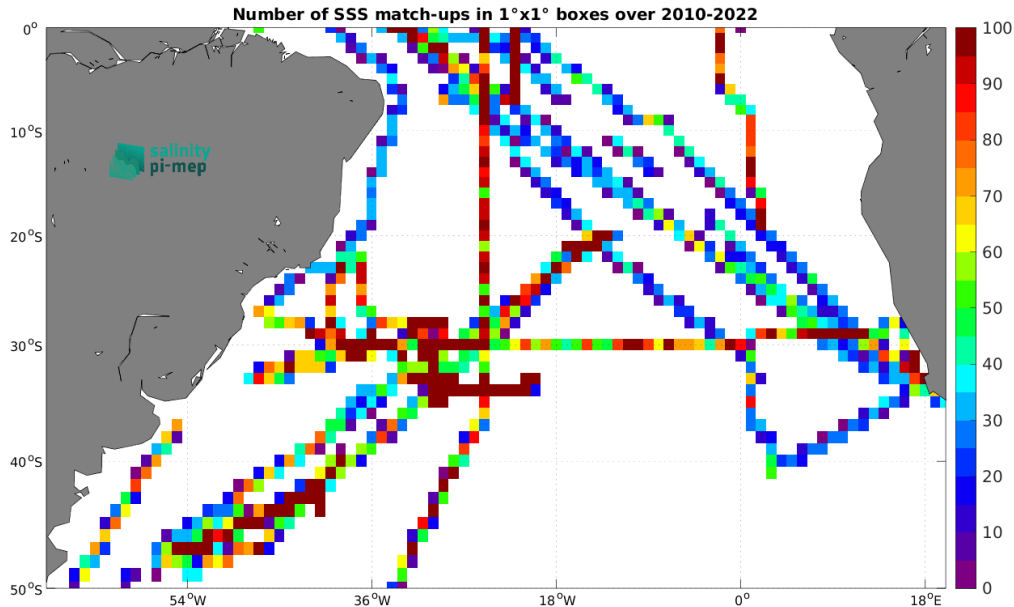
Figure 4: Number of SSS match-ups between TSG (SAMOS) SSS and the SMOS SSS L3 v8 - 18 Days (CATDS-CEC-LOCEAN) SSS product for the South Atlantic Ocean Pi-MEP region over 1^\circ \times 1^\circ boxes and for the full satellite product period.
