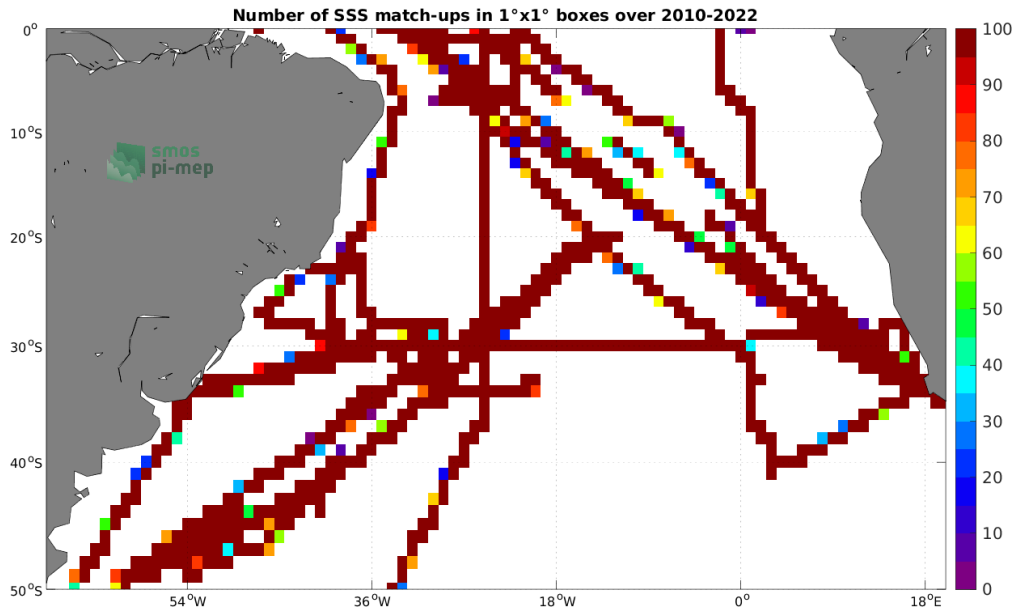
Figure 4: Number of SSS match-ups between TSG (SAMOS) SSS and the SMOS SSS L3 v8 - 18 Days (CATDS-CECOS-LOCEAN) SSS product for the South Atlantic Ocean Pi-MEP region over 1^\circ \times 1^\circ boxes and for the full satellite product period.
