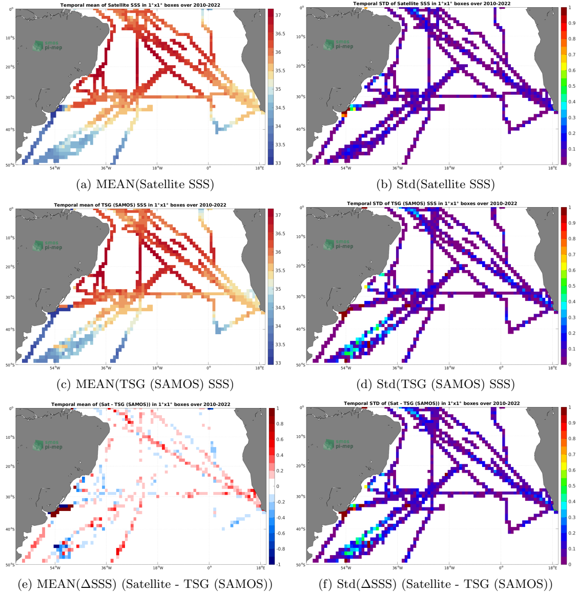
Figure 6: Temporal mean (left) and Std (right) of SSS from SMOS SSS L3 v8 - 18 Days (CATDS-CECOS-LOCEAN) (top), TSG (SAMOS) (middle), and of \Delta SSS (Satellite - TSG (SAMOS)). Only match-up pairs are used to generate these maps.
