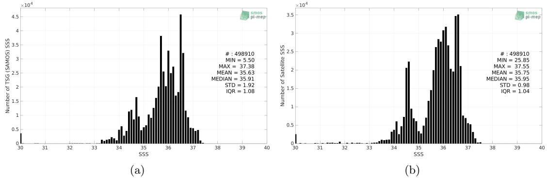
Figure 2: Histograms of SSS from TSG (SAMOS) (a) and SMOS SSS L3 v8 - 18 Days (CATDS-CECOS-LOCEAN) (b) considering all match-up pairs per bins of 0.1 over the South Atlantic Ocean Pi-MEP region and for the full satellite product period.
