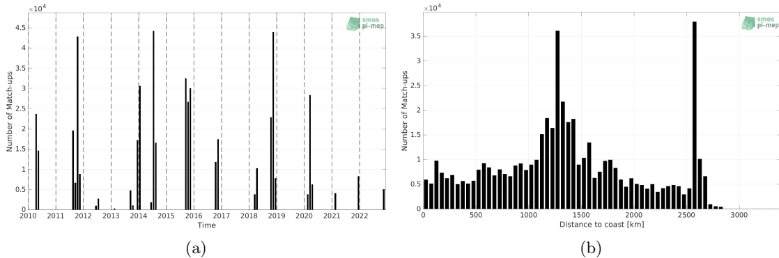
Figure 1: Number of match-ups between TSG (SAMOS) and SMOS SSS L3 v8 - 18 Days (CATDS-CECOS-LOCEAN) SSS as a function of time (a) and as function of the distance to coast (b) over the South Atlantic Ocean Pi-MEP region and for the full satellite product period.
