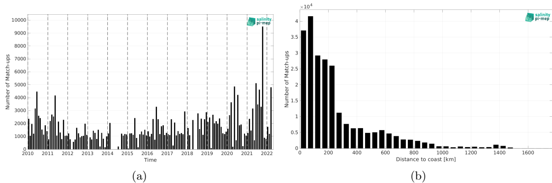
Figure 1: Number of match-ups between TSG (LEGOS-DM) and SMOS SSS L3 v8 - 18 Days (CATDS-CEC-LOCEAN) SSS as a function of time (a) and as function of the distance to coast (b) over the South Atlantic Ocean Pi-MEP region and for the full satellite product period.
