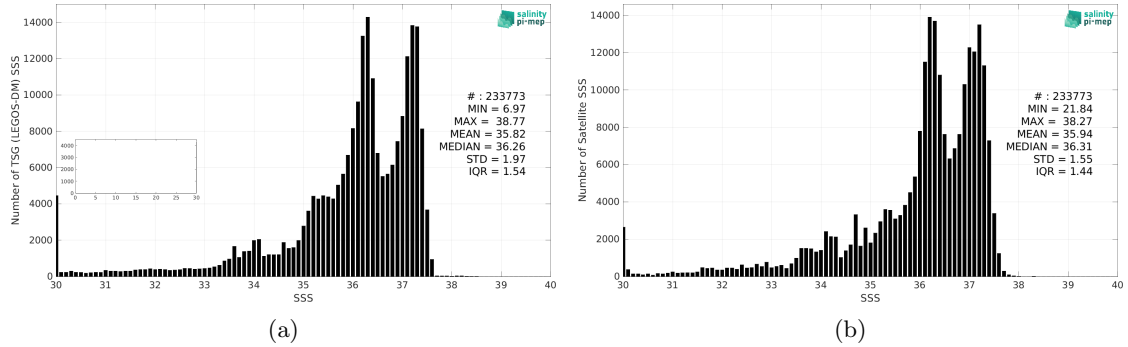
Figure 2: Histograms of SSS from TSG (LEGOS-DM) (a) and SMOS SSS L3 v8 - 18 Days (CATDS-CEC-LOCEAN) (b) considering all match-up pairs per bins of 0.1 over the South Atlantic Ocean Pi-MEP region and for the full satellite product period.
