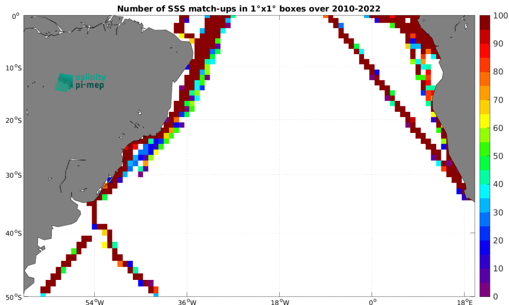
Figure 4: Number of SSS match-ups between TSG (LEGOS-DM) SSS and the SMOS SSS L3 v8 - 18 Days (CATDS-CEC-LOCEAN) SSS product for the South Atlantic Ocean Pi-MEP region over 1^\circ \times 1^\circ boxes and for the full satellite product period.
