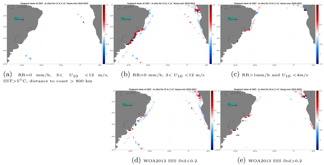
Figure 12: Temporal mean gridded over spatial boxes of size 1^\circ \times 1^\circ of \Delta SSS (SMOS SSS L3 v8 - 18 Days (CATDS-CEC-LOCEAN) - TSG (LEGOS-DM)) for 5 different subdatasets corresponding to:RR=0 mm/h, 3 < U_{10} < 12 m/s, SST >5^\circ\text{C} , distance to coast > 800 km (a), RR=0 mm/h, 3 < U_{10} < 12 m/s (b), RR >1 mm/h and U_{10} < 4 m/s (c), WOA2013 SSS Std <0.2 (d), WOA2013 SSS Std >0.2 (e).
