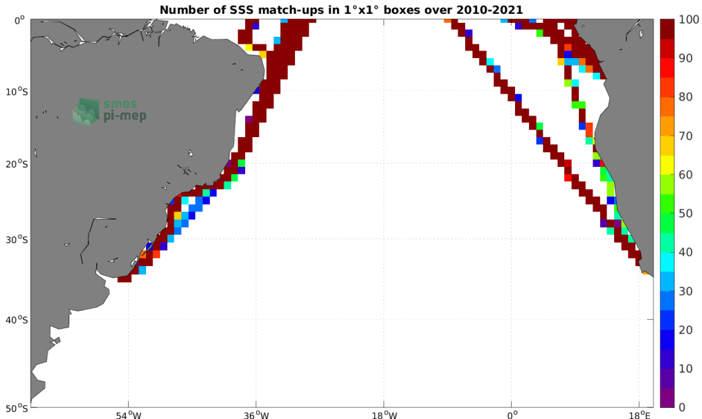
Figure 4: Number of SSS match-ups between TSG (LEGOS-DM) SSS and the SMOS SSS L3 v8 - 18 Days (CATDS-CECOS-LOCEAN) SSS product for the South Atlantic Ocean Pi-MEP region over 1^\circ \times 1^\circ boxes and for the full satellite product period.
