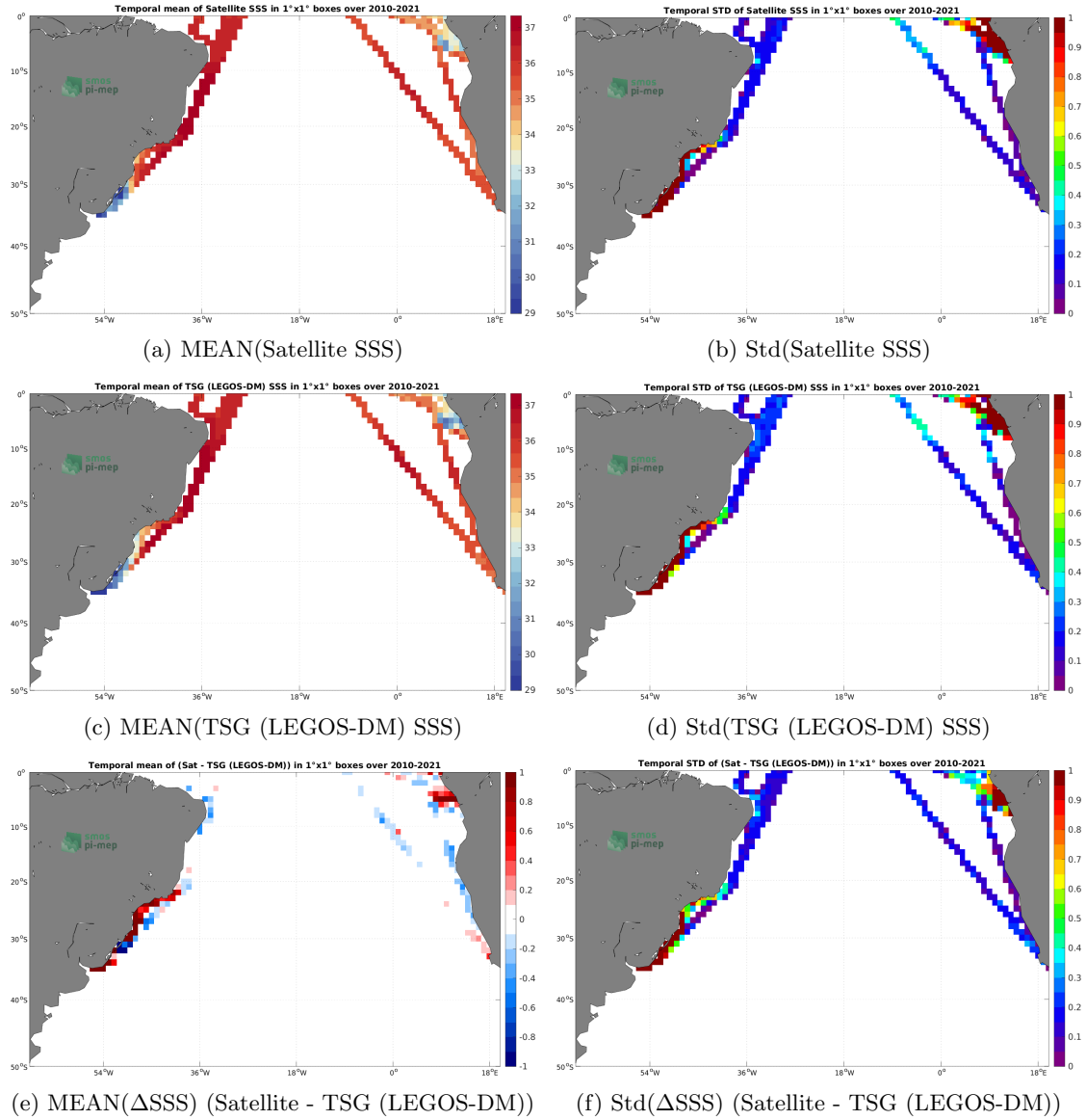
Figure 6: Temporal mean (left) and Std (right) of SSS from SMOS SSS L3 v8 - 18 Days (CATDS-CECOS-LOCEAN) (top), TSG (LEGOS-DM) ( in situ dataset (in blue)). Only match-up pairs are used to generate these maps.
