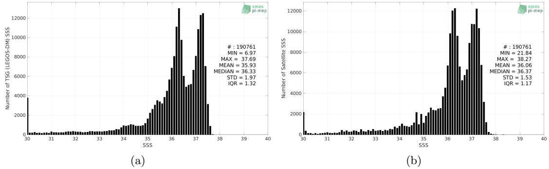
Figure 2: Histograms of SSS from TSG (LEGOS-DM) (a) and SMOS SSS L3 v8 - 18 Days (CATDS-CECOS-LOCEAN) (b) considering all match-up pairs per bins of 0.1 over the South Atlantic Ocean Pi-MEP region and for the full satellite product period.
