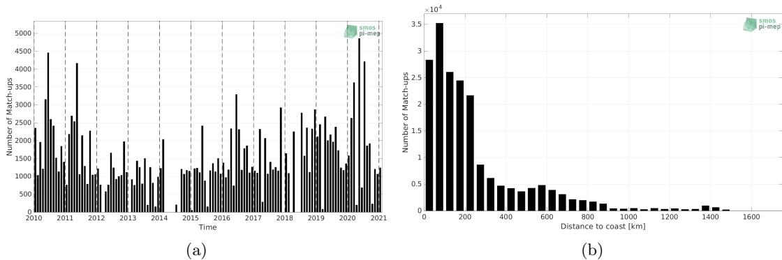
Figure 1: Number of match-ups between TSG (LEGOS-DM) and SMOS SSS L3 v8 - 18 Days (CATDS-CECOS-LOCEAN) SSS as a function of time (a) and as function of the distance to coast (b) over the South Atlantic Ocean Pi-MEP region and for the full satellite product period.
