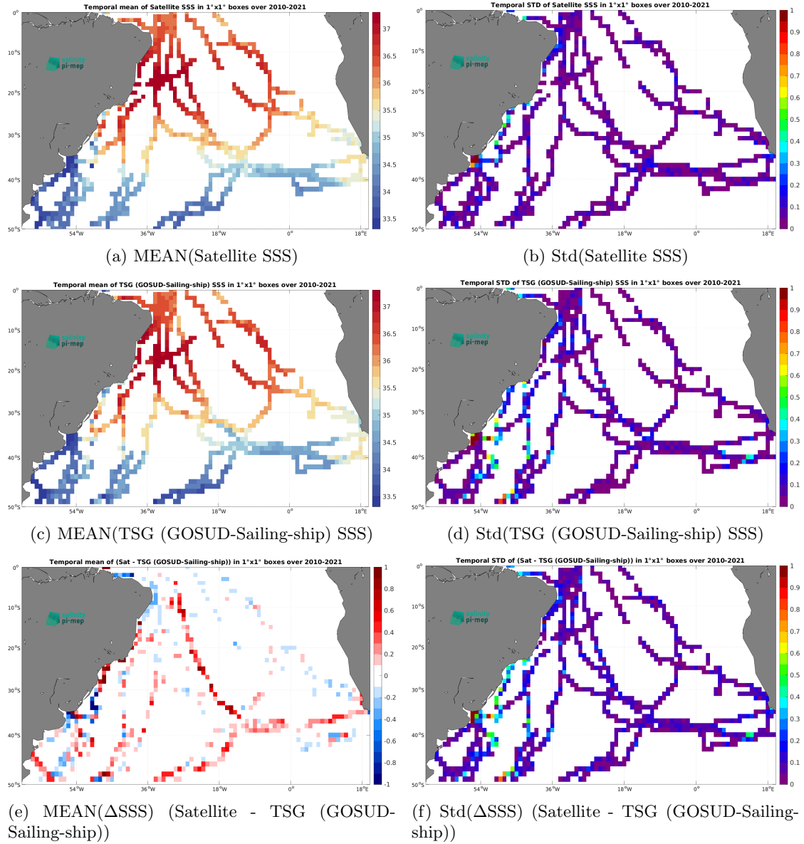
Figure 6: Temporal mean (left) and Std (right) of SSS from SMOS SSS L3 v8 - 18 Days (CATDS-CEC-LOCEAN) (top), TSG (GOSUD-Sailing-ship) (middle), and of \Delta SSS (Satellite - TSG (GOSUD-Sailing-ship)). Only match-up pairs are used to generate these maps.
