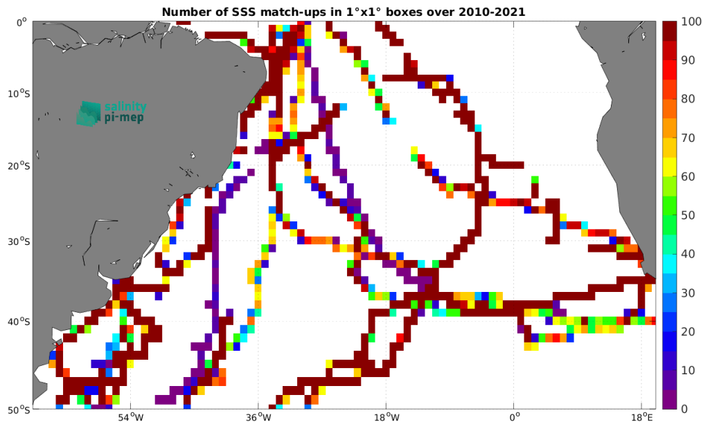
Figure 4: Number of SSS match-ups between TSG (GOSUD-Sailing-ship) SSS and the SMOS SSS L3 v8 - 18 Days (CATDS-CEC-LOCEAN) SSS product for the South Atlantic Ocean Pi-MEP region over 1^\circ \times 1^\circ boxes and for the full satellite product period.
