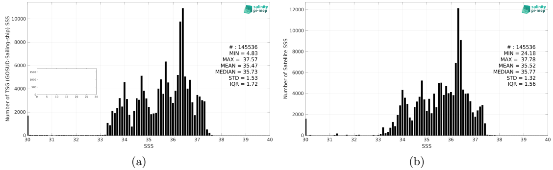
Figure 2: Histograms of SSS from TSG (GOSUD-Sailing-ship) (a) and SMOS SSS L3 v8 - 18 Days (CATDS-CEC-LOCEAN) (b) considering all match-up pairs per bins of 0.1 over the South Atlantic Ocean Pi-MEP region and for the full satellite product period.
