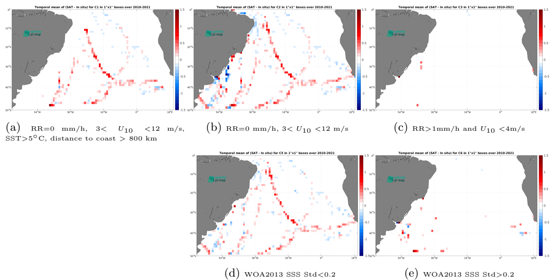
Figure 12: Temporal mean gridded over spatial boxes of size 1^\circ \times 1^\circ of \Delta SSS (SMOS SSS L3 v8 - 18 Days (CATDS-CEC-LOCEAN) - TSG (GOSUD-Sailing-ship)) for 5 different subdatasets corresponding to:RR=0 mm/h, 3 < U_{10} < 12 m/s, SST >5^\circ\text{C} , distance to coast > 800 km (a), RR=0 mm/h, 3 < U_{10} < 12 m/s (b), RR >1 mm/h and U_{10} < 4 m/s (c), WOA2013 SSS Std <0.2 (d), WOA2013 SSS Std >0.2 (e).
