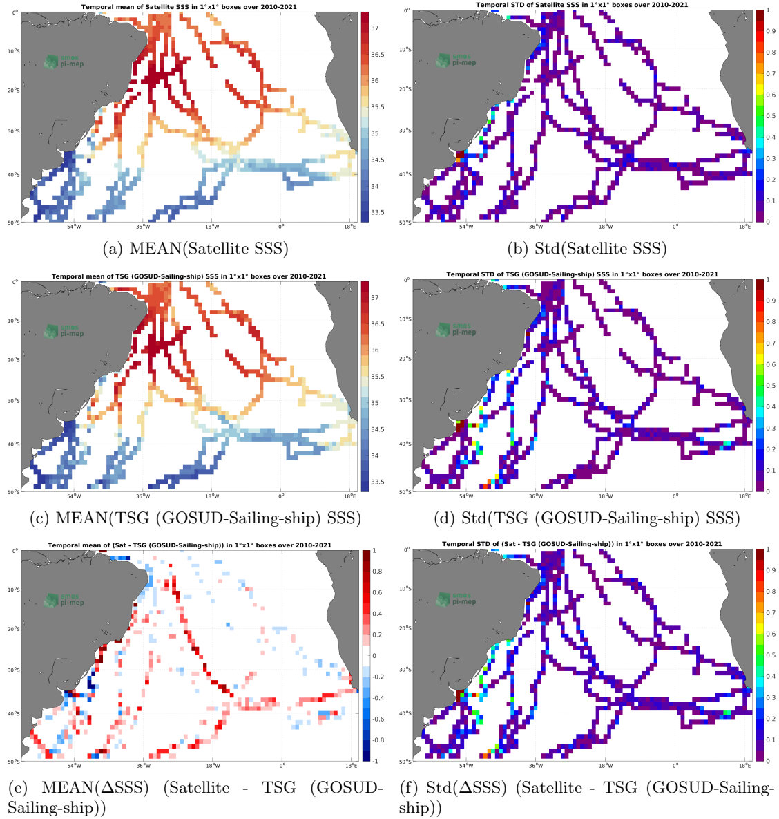
Figure 6: Temporal mean (left) and Std (right) of SSS from SMOS SSS L3 v8 - 18 Days (CATDS-CECOS-LOCEAN) (top), TSG (GOSUD-Sailing-ship) (middle), and of \Delta SSS (Satellite - TSG (GOSUD-Sailing-ship)). Only match-up pairs are used to generate these maps.
