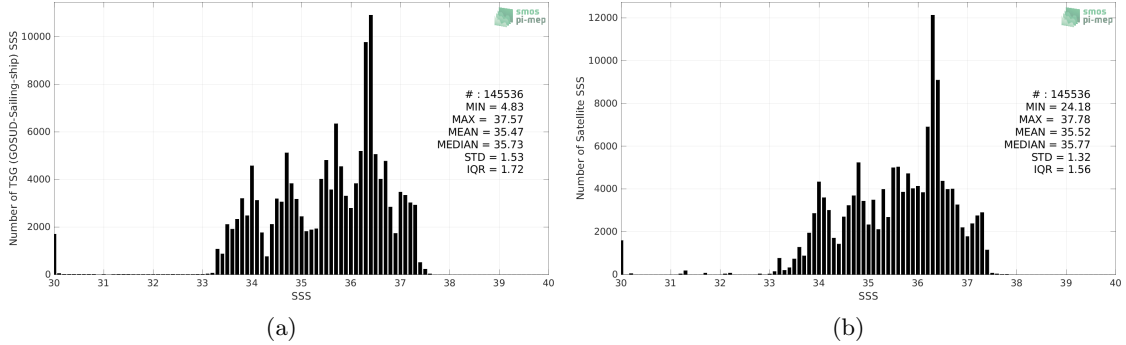
Figure 2: Histograms of SSS from TSG (GOSUD-Sailing-ship) (a) and SMOS SSS L3 v8 - 18 Days (CATDS-CECOS-LOCEAN) (b) considering all match-up pairs per bins of 0.1 over the South Atlantic Ocean Pi-MEP region and for the full satellite product period.
