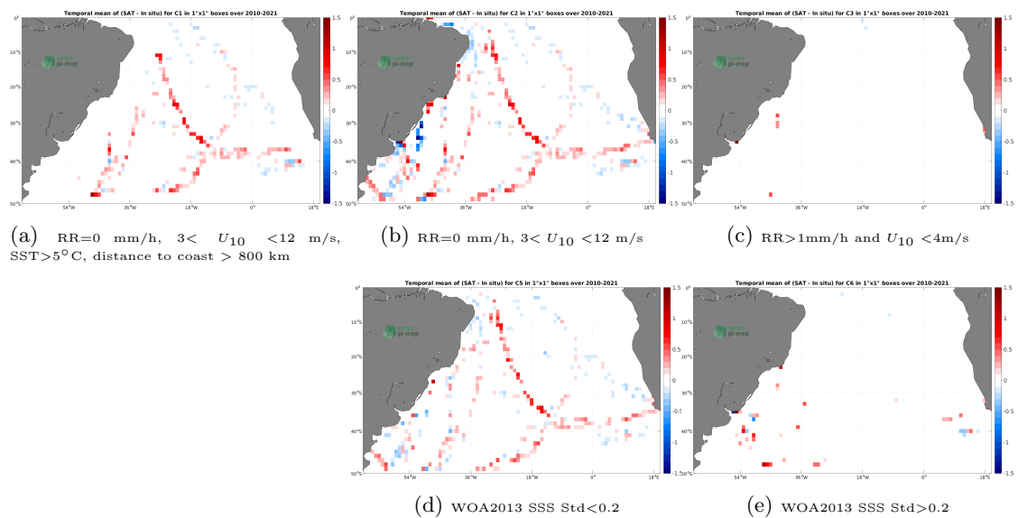
Figure 12: Temporal mean gridded over spatial boxes of size 1^\circ \times 1^\circ of \Delta\text{SSS} (SMOS SSS L3 v8 - 18 Days (CATDS-CECOS-LOCEAN) - TSG (GOSUD-Sailing-ship)) for 5 different subdatasets corresponding to:RR=0 mm/h, 3 < U_{10} < 12 m/s, SST >5^\circ\text{C} , distance to coast > 800 km (a), RR=0 mm/h, 3 < U_{10} < 12 m/s (b), RR >1 mm/h and U_{10} < 4 m/s (c), WOA2013 SSS Std <0.2 (d), WOA2013 SSS Std >0.2 (e).
