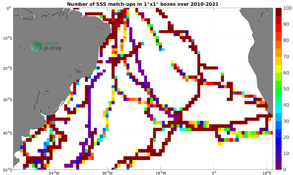
Figure 4: Number of SSS match-ups between TSG (GOSUD-Sailing-ship) SSS and the SMOS SSS L3 v8 - 18 Days (CATDS-CECOS-LOCEAN) SSS product for the South Atlantic Ocean Pi-MEP region over 1^\circ \times 1^\circ boxes and for the full satellite product period.
