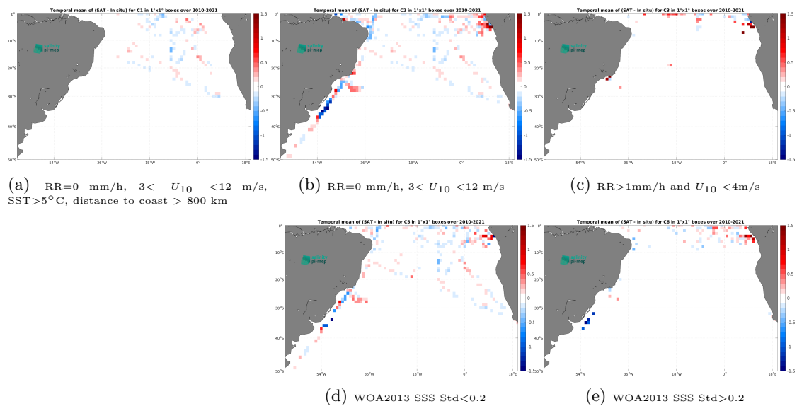
Figure 12: Temporal mean gridded over spatial boxes of size 1^\circ \times 1^\circ of \Delta\text{SSS} (SMOS SSS L3 v8 - 18 Days (CATDS-CEC-LOCEAN) - TSG (GOSUD-Research-vessel)) for 5 different subdatasets corresponding to:RR=0 mm/h, 3 < U_{10} < 12 m/s, SST >5^\circ\text{C} , distance to coast > 800 km (a), RR=0 mm/h, 3 < U_{10} < 12 m/s (b), RR >1 mm/h and U_{10} < 4 m/s (c), WOA2013 SSS Std <0.2 (d), WOA2013 SSS Std >0.2 (e).
