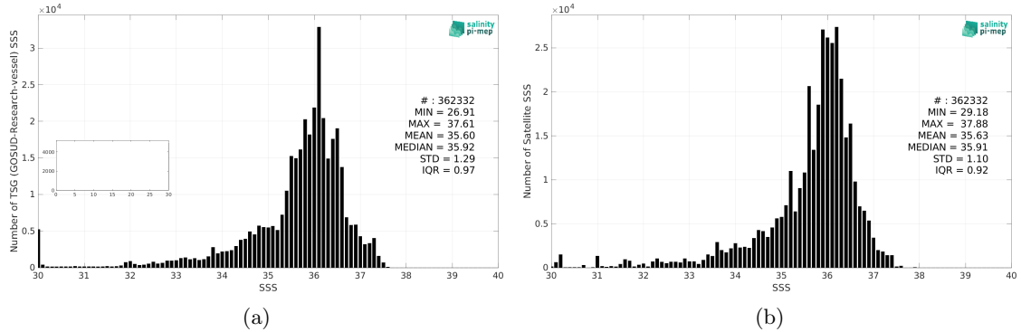
Figure 2: Histograms of SSS from TSG (GOSUD-Research-vessel) (a) and SMOS SSS L3 v8 - 18 Days (CATDS-CEC-LOCEAN) (b) considering all match-up pairs per bins of 0.1 over the South Atlantic Ocean Pi-MEP region and for the full satellite product period.
