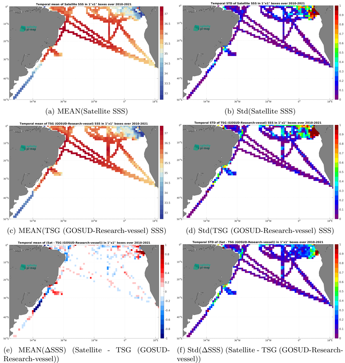
Figure 6: Temporal mean (left) and Std (right) of SSS from SMOS SSS L3 v8 - 18 Days (CATDS-CEC-LOCEAN) (top), TSG (GOSUD-Research-vessel) (middle), and of \Delta SSS (Satellite - TSG (GOSUD-Research-vessel)). Only match-up pairs are used to generate these maps.
