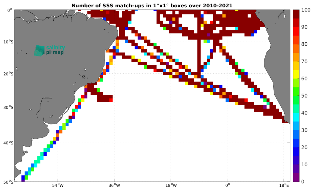
Figure 4: Number of SSS match-ups between TSG (GOSUD-Research-vessel) SSS and the SMOS SSS L3 v8 - 18 Days (CATDS-CEC-LOCEAN) SSS product for the South Atlantic Ocean Pi-MEP region over 1^\circ \times 1^\circ boxes and for the full satellite product period.
