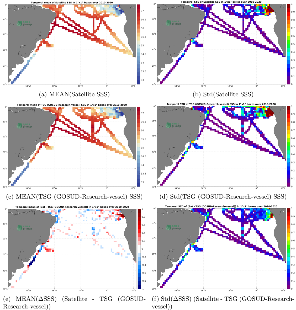
Figure 6: Temporal mean (left) and Std (right) of SSS from SMOS SSS L3 v8 - 18 Days (CATDS-CECOS-LOCEAN) (top), TSG (GOSUD-Research-vessel) (middle), and of \Delta SSS (Satellite - TSG (GOSUD-Research-vessel)). Only match-up pairs are used to generate these maps.
