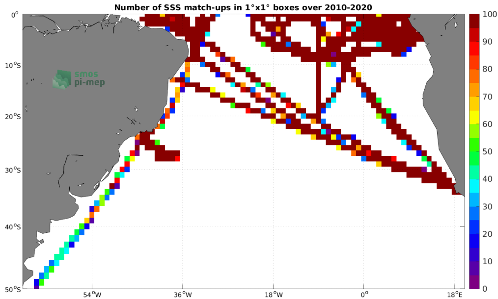
Figure 4: Number of SSS match-ups between TSG (GOSUD-Research-vessel) SSS and the SMOS SSS L3 v8 - 18 Days (CATDS-CECOS-LOCEAN) SSS product for the South Atlantic Ocean Pi-MEP region over 1^\circ \times 1^\circ boxes and for the full satellite product period.
