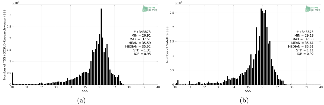
Figure 2: Histograms of SSS from TSG (GOSUD-Research-vessel) (a) and SMOS SSS L3 v8 - 18 Days (CATDS-CECOS-LOCEAN) (b) considering all match-up pairs per bins of 0.1 over the South Atlantic Ocean Pi-MEP region and for the full satellite product period.
