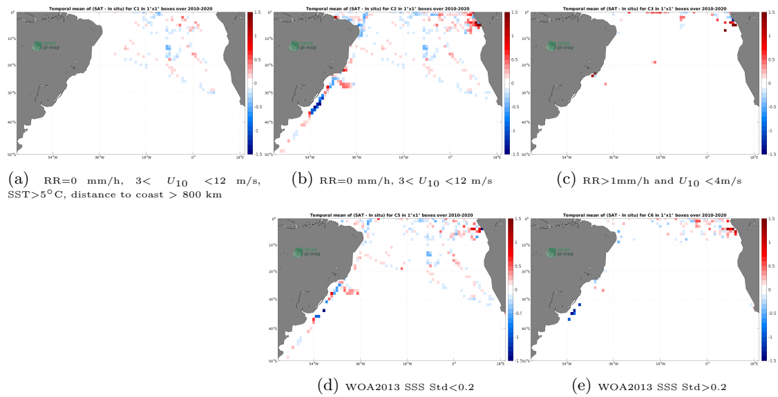
Figure 12: Temporal mean gridded over spatial boxes of size 1^\circ \times 1^\circ of \Delta SSS (SMOS SSS L3 v8 - 18 Days (CATDS-CECOS-LOCEAN) - TSG (GOSUD-Research-vessel)) for 5 different sub-datasets corresponding to:RR=0 mm/h, 3 < U_{10} < 12 m/s, SST >5^\circ\text{C} , distance to coast > 800 km (a), RR=0 mm/h, 3 < U_{10} < 12 m/s (b), RR >1 mm/h and U_{10} < 4 m/s (c), WOA2013 SSS Std <0.2 (d), WOA2013 SSS Std >0.2 (e).
