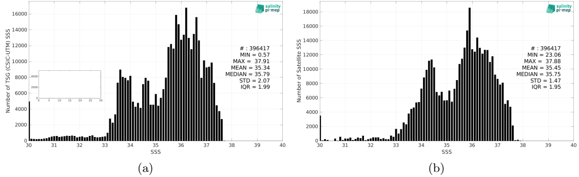
Figure 2: Histograms of SSS from TSG (CSIC-UTM) (a) and SMOS SSS L3 v8 - 18 Days (CATDS-CEC-LOCEAN) (b) considering all match-up pairs per bins of 0.1 over the South Atlantic Ocean Pi-MEP region and for the full satellite product period.
