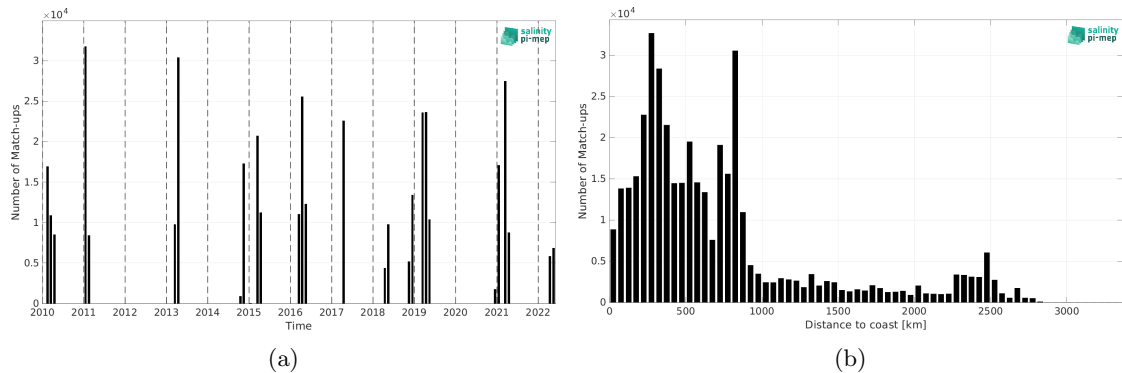
Figure 1: Number of match-ups between TSG (CSIC-UTM) and SMOS SSS L3 v8 - 18 Days (CATDS-CEC-LOCEAN) SSS as a function of time (a) and as function of the distance to coast (b) over the South Atlantic Ocean Pi-MEP region and for the full satellite product period.
