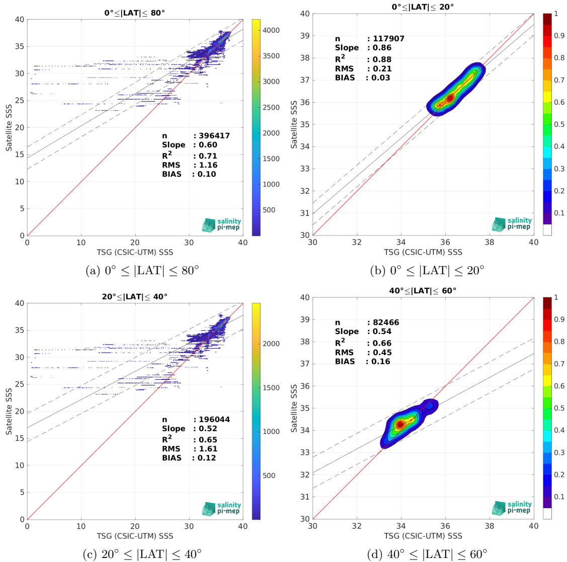
Figure 9: Contour maps of the concentration of SMOS SSS L3 v8 - 18 Days (CATDS-CEC-LOCEAN) SSS ( y -axis) versus TSG (CSIC-UTM) SSS ( x -axis) at match-up pairs for different latitude bands. For each plot, the red line shows x=y . The black thin and dashed lines indicate a linear fit through the data cloud and the \pm 95\% confidence levels, respectively. The number match-up pairs n , the slope and R^2 coefficient of the linear fit, the root mean square (RMS) and the mean bias between satellite and in situ data are indicated for each latitude band in each plots.
