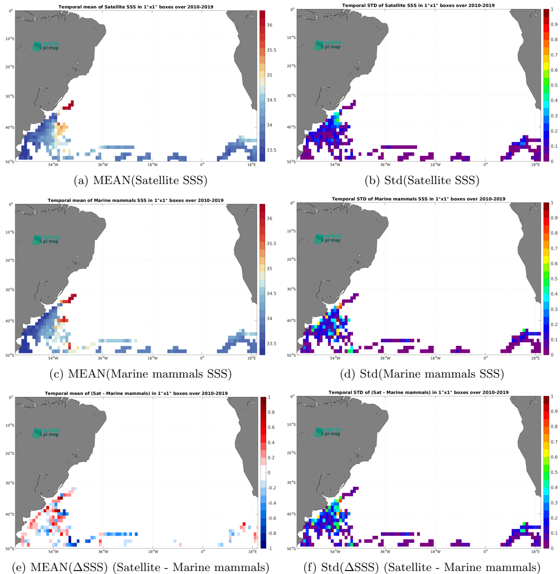
Figure 6: Temporal mean (left) and Std (right) of SSS from SMOS SSS L3 v8 - 18 Days (CATDS-CEC-LOCEAN) (top), Marine mammals (middle), and of \Delta SSS (Satellite - Marine mammals). Only match-up pairs are used to generate these maps.
