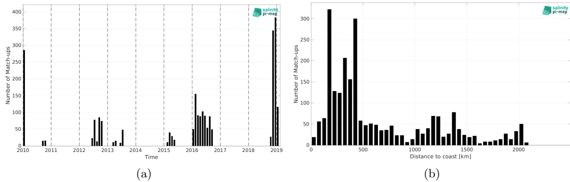
Figure 1: Number of match-ups between Marine mammals and SMOS SSS L3 v8 - 18 Days (CATDS-CEC-LOCEAN) SSS as a function of time (a) and as function of the distance to coast (b) over the South Atlantic Ocean Pi-MEP region and for the full satellite product period.
