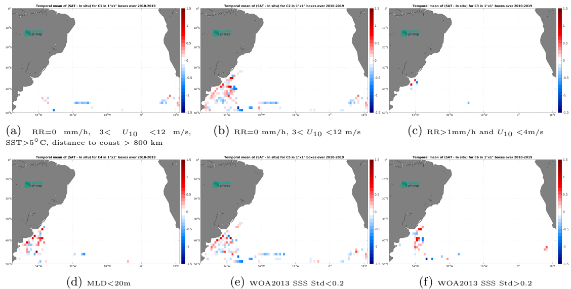
Figure 12: Temporal mean gridded over spatial boxes of size 1^{\circ}\times 1^{\circ} of \Delta\text{SSS} (SMOS SSS L3 v8 - 18 Days (CATDS-CEC-LOCEAN) - Marine mammals) for 6 different subdatasets corresponding to:RR=0 mm/h, 3 < U_{10} < 12 m/s, SST >5^{\circ}\text{C} , distance to coast > 800 km (a), RR=0 mm/h, 3 < U_{10} < 12 m/s (b), RR >1 mm/h and U_{10} < 4 m/s (c),MLD <20 m (d),WOA2013 SSS Std <0.2 (e),WOA2013 SSS Std >0.2 (f).
