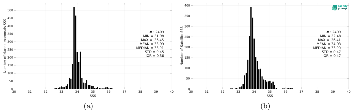
Figure 2: Histograms of SSS from Marine mammals (a) and SMOS SSS L3 v8 - 18 Days (CATDS-CEC-LOCEAN) (b) considering all match-up pairs per bins of 0.1 over the South Atlantic Ocean Pi-MEP region and for the full satellite product period.
