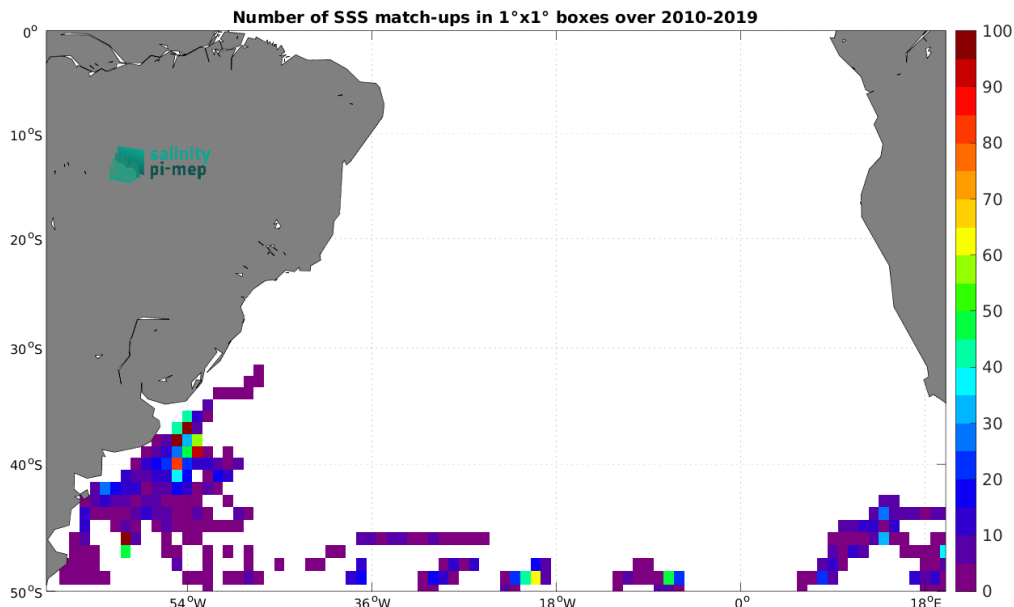
Figure 4: Number of SSS match-ups between Marine mammals SSS and the SMOS SSS L3 v8 - 18 Days (CATDS-CEC-LOCEAN) SSS product for the South Atlantic Ocean Pi-MEP region over 1^\circ \times 1^\circ boxes and for the full satellite product period.
