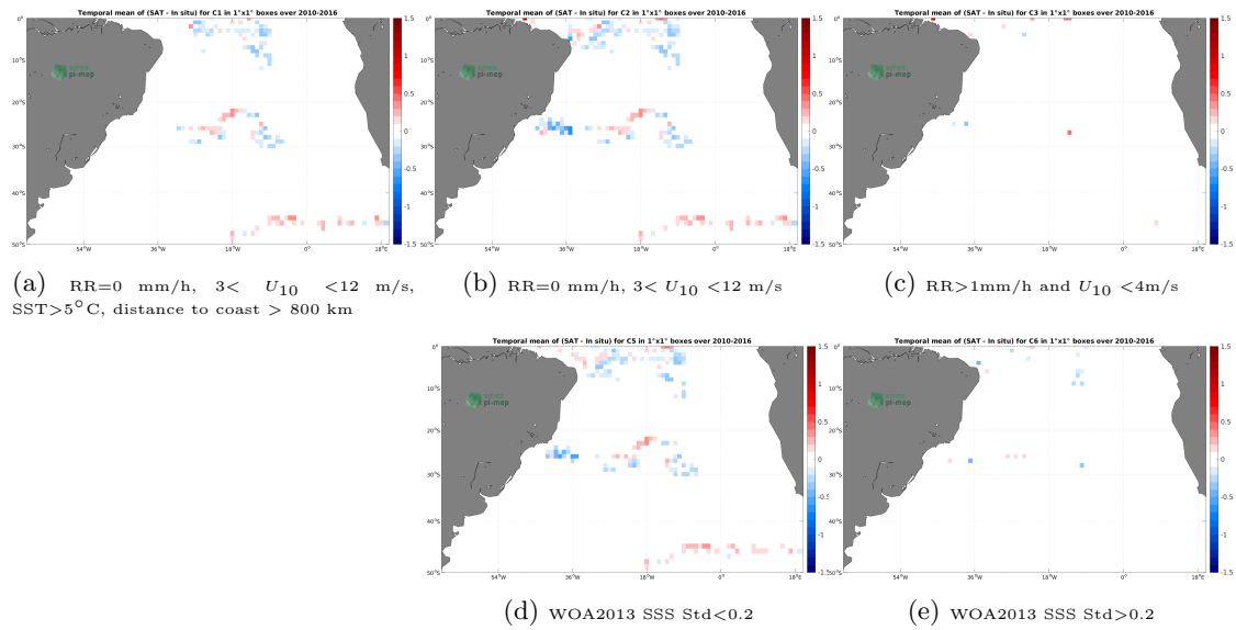
Figure 11: Temporal mean gridded over spatial boxes of size 1^\circ \times 1^\circ of \Delta\text{SSS} (SMOS SSS L3 v8 - 18 Days (CATDS-CECOS-LOCEAN) - Surface drifters) for 5 different subdatasets corresponding to:RR=0 mm/h, 3 < U_{10} < 12 m/s, SST >5^\circ\text{C} , distance to coast > 800 km (a), RR=0 mm/h, 3 < U_{10} < 12 m/s (b), RR >1 mm/h and U_{10} < 4 m/s (c), WOA2013 SSS Std <0.2 (d), WOA2013 SSS Std >0.2 (e).
