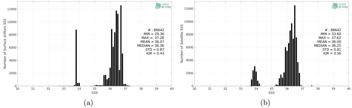
Figure 2: Histograms of SSS from Surface drifters (a) and SMOS SSS L3 v8 - 18 Days (CATDS-CECOS-LOCEAN) (b) considering all match-up pairs per bins of 0.1 over the South Atlantic Ocean Pi-MEP region and for the full satellite product period.
