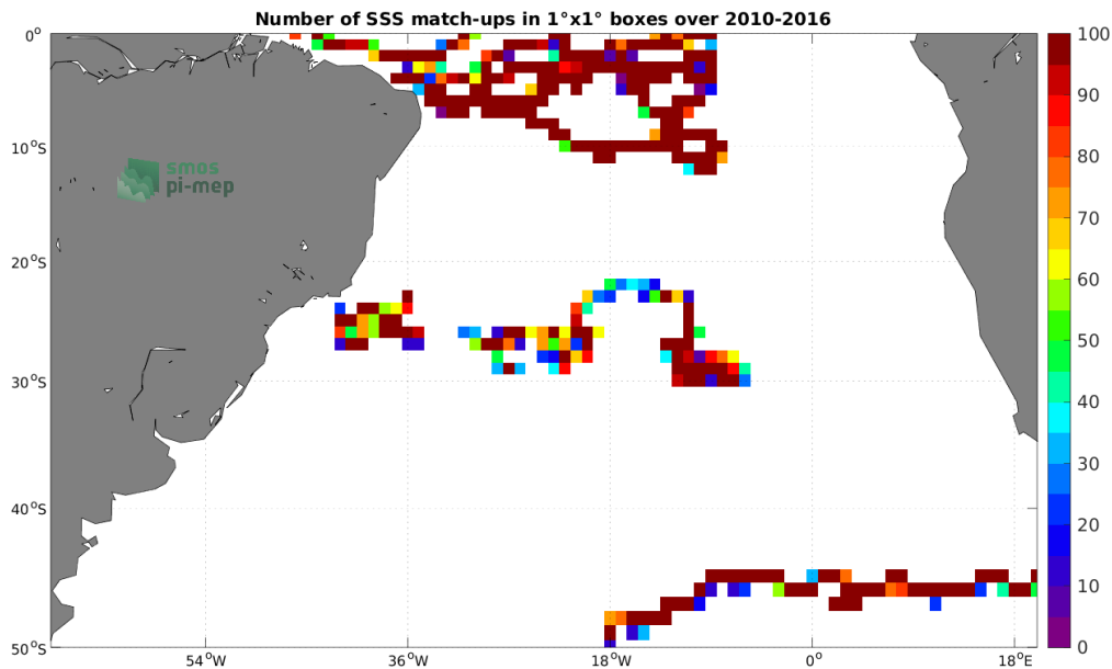
Figure 3: Number of SSS match-ups between Surface drifters SSS and the SMOS SSS L3 v8 - 18 Days (CATDS-CECOS-LOCEAN) SSS product for the South Atlantic Ocean Pi-MEP region over 1^\circ \times 1^\circ boxes and for the full satellite product period.
