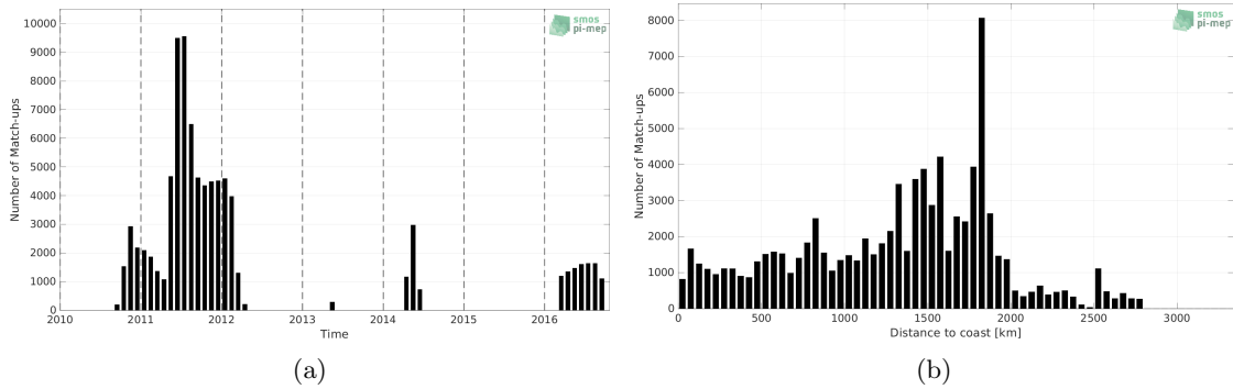
Figure 1: Number of match-ups between Surface drifters and SMOS SSS L3 v8 - 18 Days (CATDS-CECOS-LOCEAN) SSS as a function of time (a) and as function of the distance to coast (b) over the South Atlantic Ocean Pi-MEP region and for the full satellite product period.
