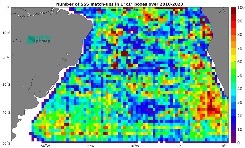
Figure 4: Number of SSS match-ups between Argo SSS and the SMOS SSS L3 v8 - 18 Days (CATDS-CEC-LOCEAN) SSS product for the South Atlantic Ocean Pi-MEP region over 1^\circ \times 1^\circ boxes and for the full satellite product period.
