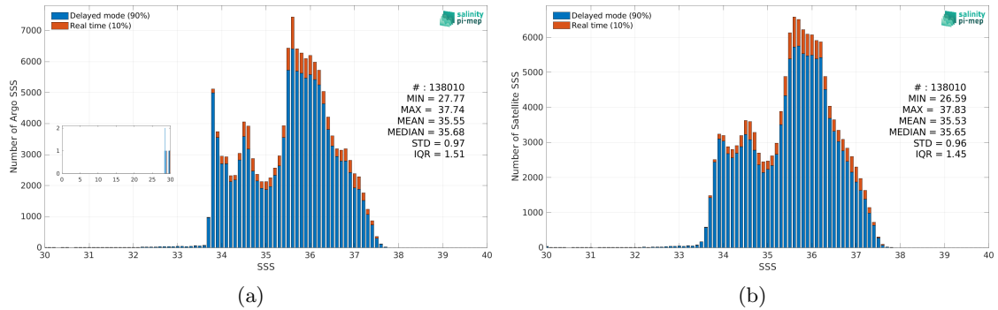
Figure 2: Histograms of SSS from Argo (a) and SMOS SSS L3 v8 - 18 Days (CATDS-CEC-LOCEAN) (b) considering all match-up pairs per bins of 0.1 over the South Atlantic Ocean Pi-MEP region and for the full satellite product period.
