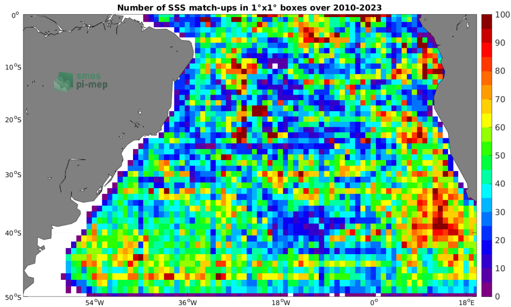
Figure 4: Number of SSS match-ups between Argo SSS and the SMOS SSS L3 v8 - 18 Days (CATDS-CECOS-LOCEAN) SSS product for the South Atlantic Ocean Pi-MEP region over 1^\circ \times 1^\circ boxes and for the full satellite product period.
