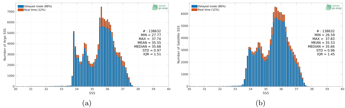
Figure 2: Histograms of SSS from Argo (a) and SMOS SSS L3 v8 - 18 Days (CATDS-CECOS-LOCEAN) (b) considering all match-up pairs per bins of 0.1 over the South Atlantic Ocean Pi-MEP region and for the full satellite product period.
