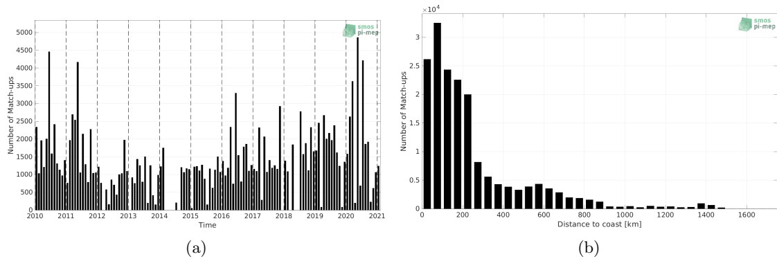
Figure 1: Number of match-ups between TSG (LEGOS-DM) and SMOS SSS L3 v7 - 9 Days (CATDS-CECOS-LOCEAN) SSS as a function of time (a) and as function of the distance to coast (b) over the South Atlantic Ocean Pi-MEP region and for the full satellite product period.
