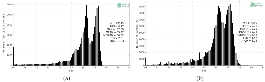
Figure 2: Histograms of SSS from TSG (LEGOS-DM) (a) and SMOS SSS L3 v7 - 9 Days (CATDS-CECOS-LOCEAN) (b) considering all match-up pairs per bins of 0.1 over the South Atlantic Ocean Pi-MEP region and for the full satellite product period.
