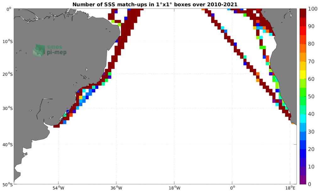
Figure 4: Number of SSS match-ups between TSG (LEGOS-DM) SSS and the SMOS SSS L3 v7 - 9 Days (CATDS-CECOS-LOCEAN) SSS product for the South Atlantic Ocean Pi-MEP region over 1^\circ \times 1^\circ boxes and for the full satellite product period.
