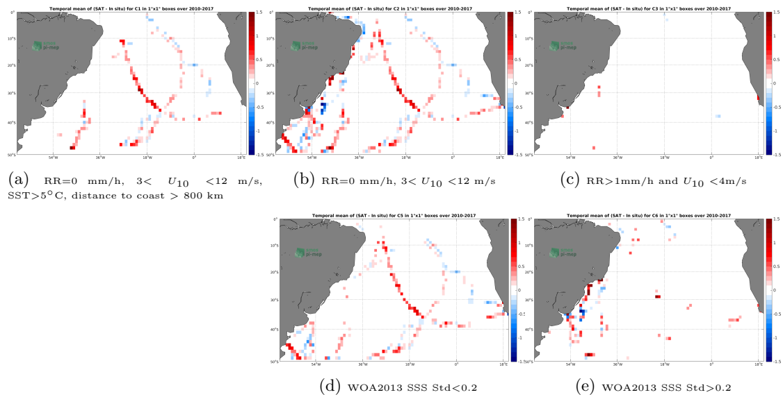
Figure 12: Temporal mean gridded over spatial boxes of size 1^\circ \times 1^\circ of \Delta SSS (SMOS SSS L3 v7 - 9 Days (CATDS-CECOS-LOCEAN) - TSG (GOSUD-Sailing-ship)) for 5 different subdatasets corresponding to: RR=0 mm/h, 3 < U_{10} < 12 m/s, SST > 5°C, distance to coast > 800 km (a), RR=0 mm/h, 3 < U_{10} < 12 m/s (b), RR > 1mm/h and U_{10} < 4 m/s (c), WOA2013 SSS Std < 0.2 (d), WOA2013 SSS Std > 0.2 (e).
