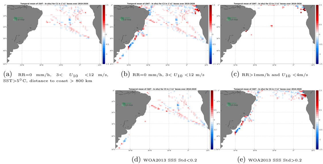
Figure 12: Temporal mean gridded over spatial boxes of size 1^\circ \times 1^\circ of \Delta SSS (SMOS SSS L3 v7 - 9 Days (CATDS-CECOS-LOCEAN) - TSG (GOSUD-Research-vessel)) for 5 different subdatasets corresponding to: RR=0 mm/h, 3 < U_{10} < 12 m/s, SST > 5°C, distance to coast > 800 km (a), RR=0 mm/h, 3 < U_{10} < 12 m/s (b), RR > 1mm/h and U_{10} < 4 m/s (c), WOA2013 SSS Std < 0.2 (d), WOA2013 SSS Std > 0.2 (e).
