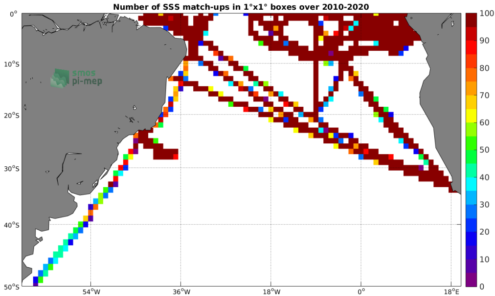
Figure 4: Number of SSS match-ups between TSG (GOSUD-Research-vessel) SSS and the SMOS SSS L3 v7 - 9 Days (CATDS-CECOS-LOCEAN) SSS product for the South Atlantic Ocean Pi-MEP region over 1^{\circ} \times 1^{\circ} boxes and for the full satellite product period.
