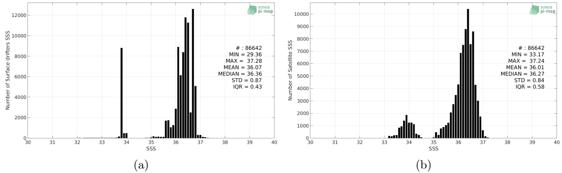
Figure 2: Histograms of SSS from Surface drifters (a) and SMOS SSS L3 v7 - 9 Days (CATDS-CECOS-LOCEAN) (b) considering all match-up pairs per bins of 0.1 over the South Atlantic Ocean Pi-MEP region and for the full satellite product period.
