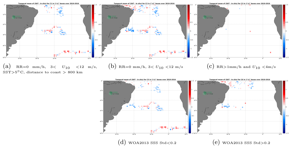
Figure 11: Temporal mean gridded over spatial boxes of size 1^\circ \times 1^\circ of \Delta SSS (SMOS SSS L3 v7 - 9 Days (CATDS-CECOS-LOCEAN) - Surface drifters) for 5 different subdatasets corresponding to: RR=0 mm/h, 3 < U_{10} < 12 m/s, SST > 5°C, distance to coast > 800 km (a), RR=0 mm/h, 3 < U_{10} < 12 m/s (b), RR > 1mm/h and U_{10} < 4 m/s (c), WOA2013 SSS Std < 0.2 (d), WOA2013 SSS Std > 0.2 (e).
