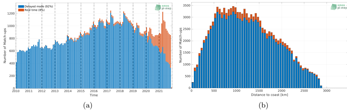
Figure 1: Number of match-ups between Argo and SMOS SSS L3 v7 - 9 Days (CATDS-CECOS-LOCEAN) SSS as a function of time (a) and as function of the distance to coast (b) over the South Atlantic Ocean Pi-MEP region and for the full satellite product period.
