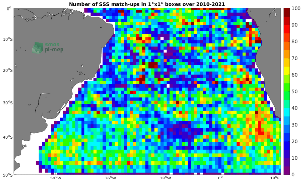
Figure 4: Number of SSS match-ups between Argo SSS and the SMOS SSS L3 v7 - 9 Days (CATDS-CECOS-LOCEAN) SSS product for the South Atlantic Ocean Pi-MEP region over 1^\circ \times 1^\circ boxes and for the full satellite product period.
