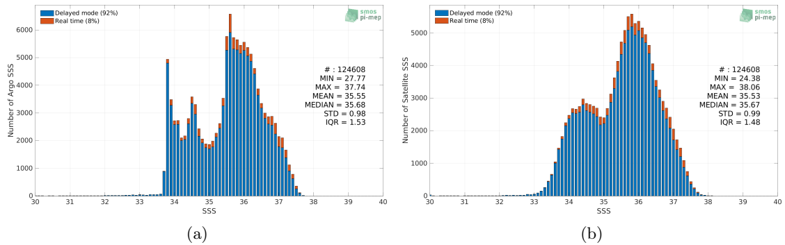
Figure 2: Histograms of SSS from Argo (a) and SMOS SSS L3 v7 - 9 Days (CATDS-CECOS-LOCEAN) (b) considering all match-up pairs per bins of 0.1 over the South Atlantic Ocean Pi-MEP region and for the full satellite product period.
